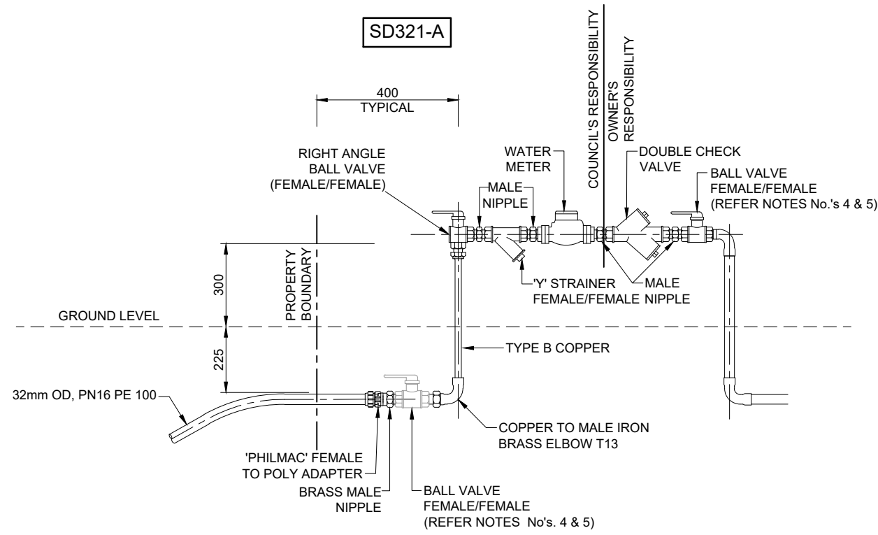
20/25mm COMMERCIAL/INDUSTRIAL WATER METER NO FIRE HOSE REELS LOW TO MEDIUM BACKFLOW HAZARD RATING
