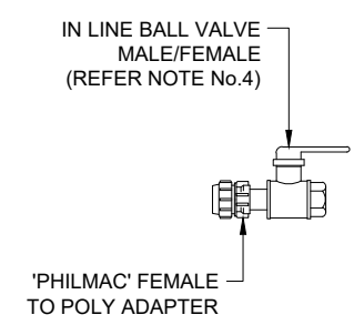
DETAIL - MALE/FEMALE BALL VALVE
