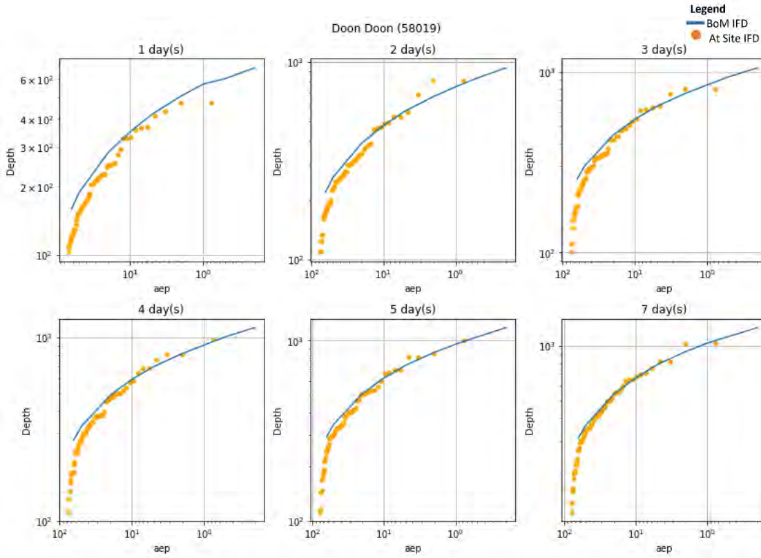
Diagram 133: Rainfall Comparison at the Doon Doon – Long Duration
