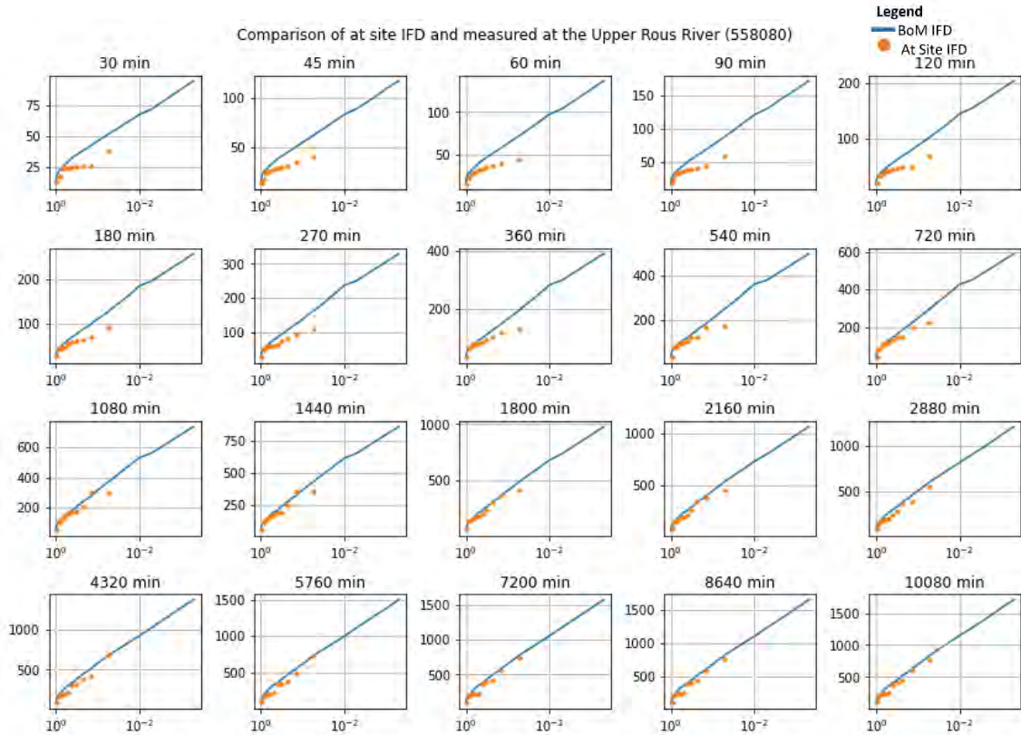
Diagram 131: Rainfall Comparison at the Upper Rous River Gauge
