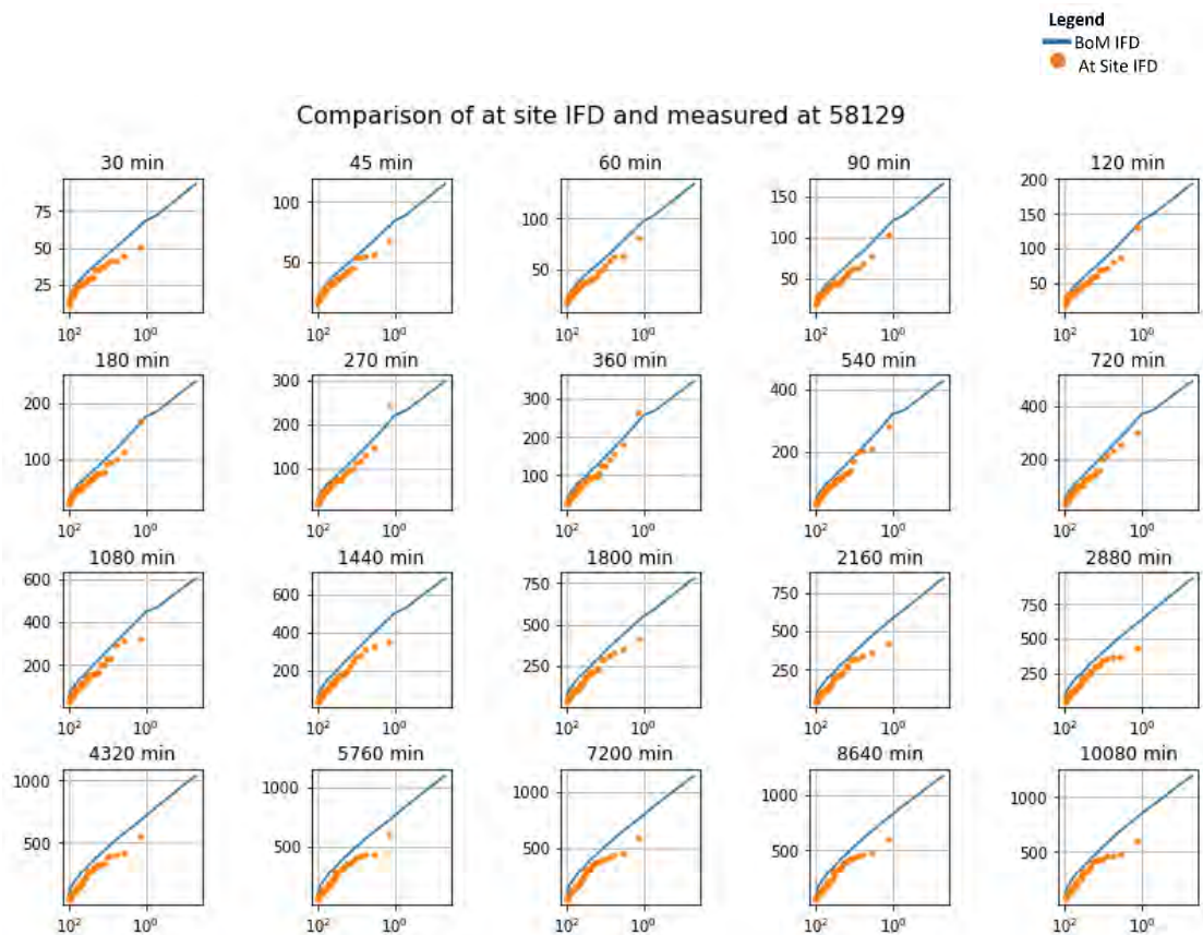
Diagram 127: Rainfall Comparison at Morning View
