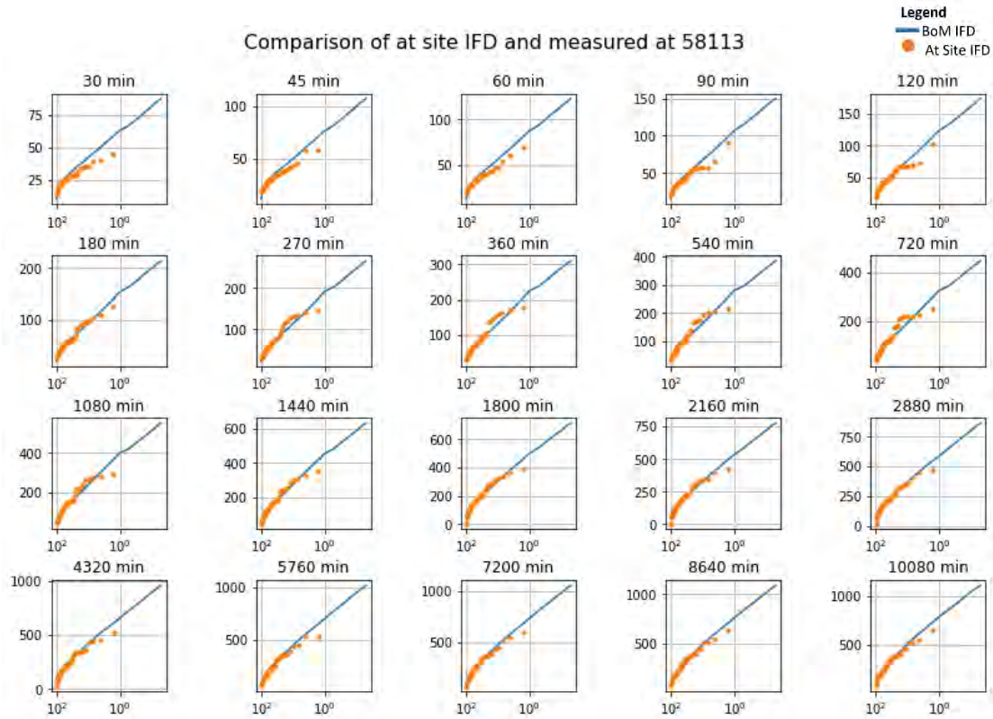
Diagram 127: Rainfall Comparison at Morning View
