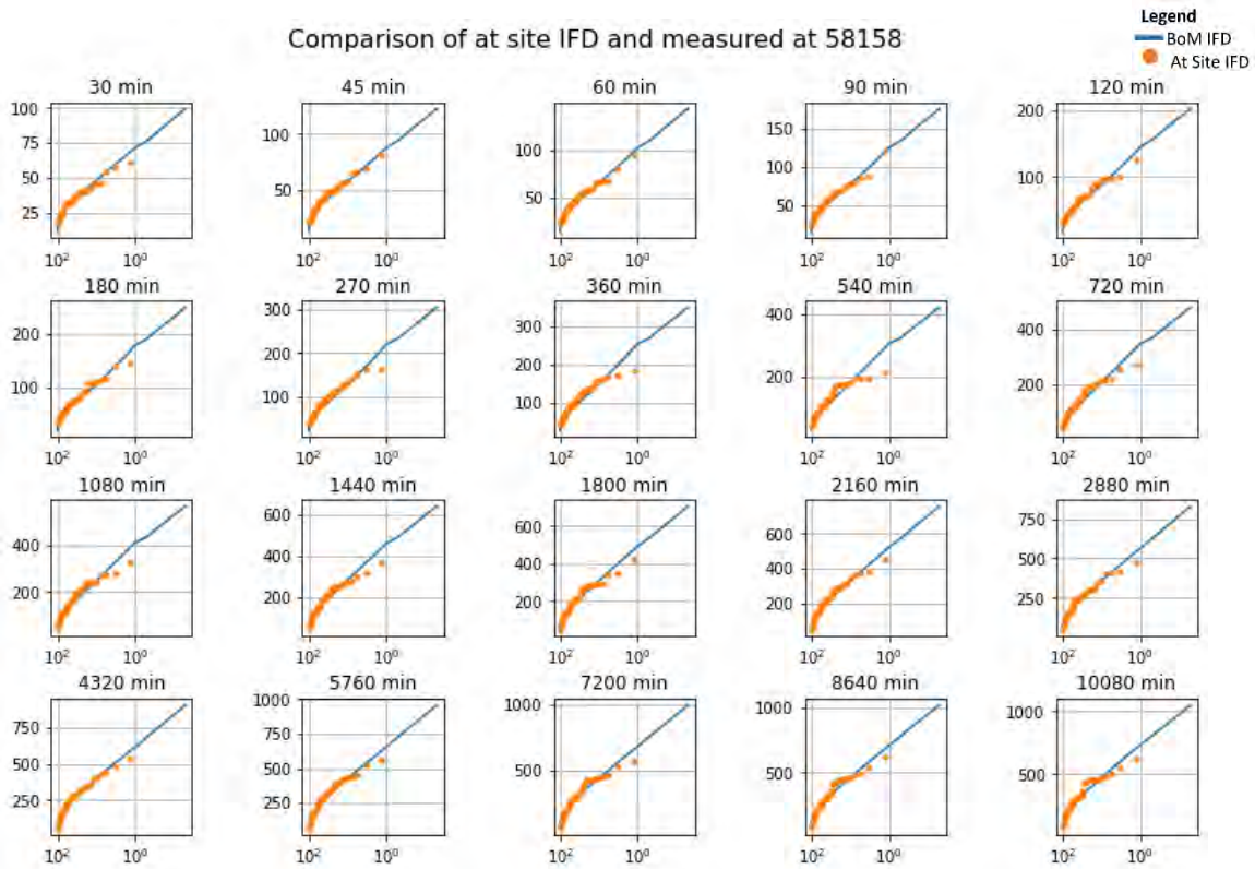
Diagram 129: Rainfall Comparison at Bray Park
