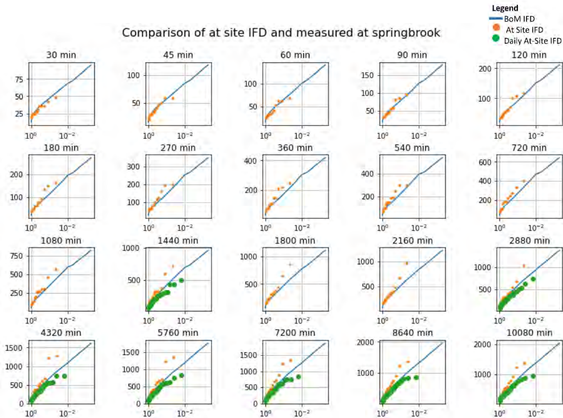
Diagram 130: Rainfall Comparison at Springbrook National Park Gauge
