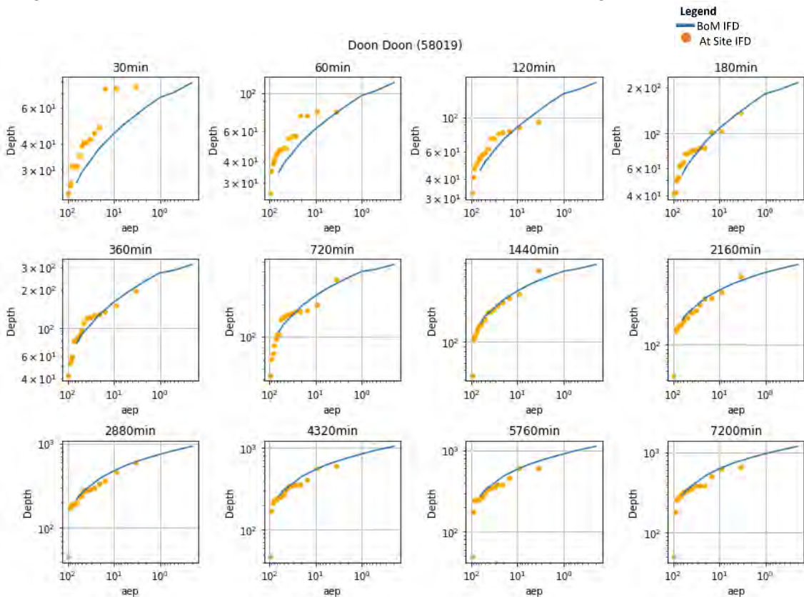
Diagram 132: Rainfall Comparison at the Doon Doon
