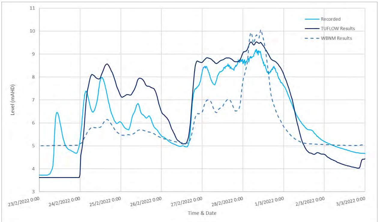
Diagram 83: 2022 Comparison of Water Level at Boat Harbour
