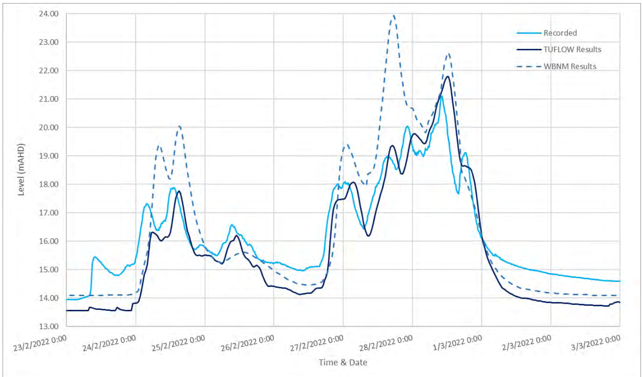
Diagram 82: 2022 Comparison of Water Level at Eungella
