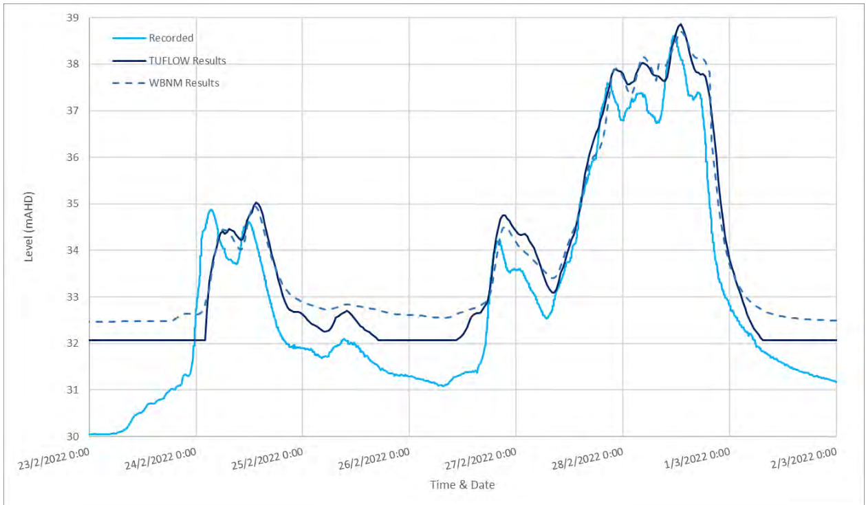
Figure 37: 2022 Comparison of Water Level at Palmers Road
