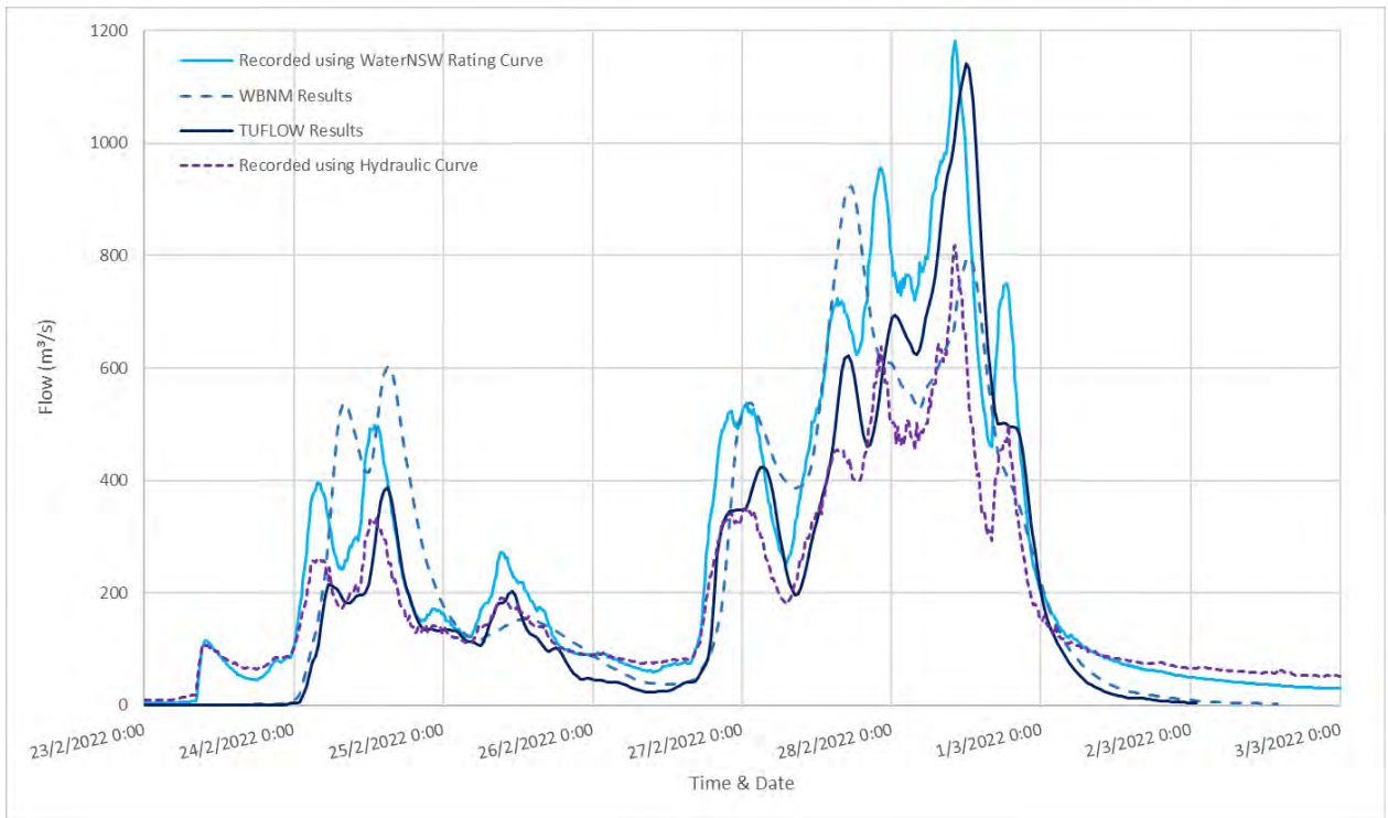
Diagram 78: 2022 Comparison of Flow at Eungella
