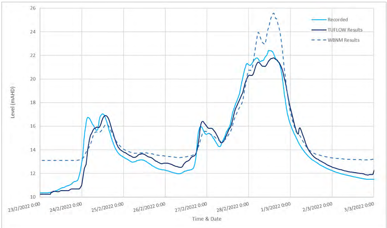
Diagram 81: 2022 Comparison of Water Level at Uki
