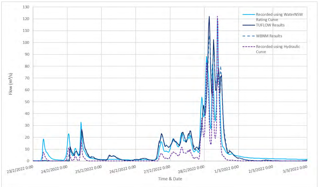
Diagram 80: 2022 Comparison of Flow at Cobaki Creek
