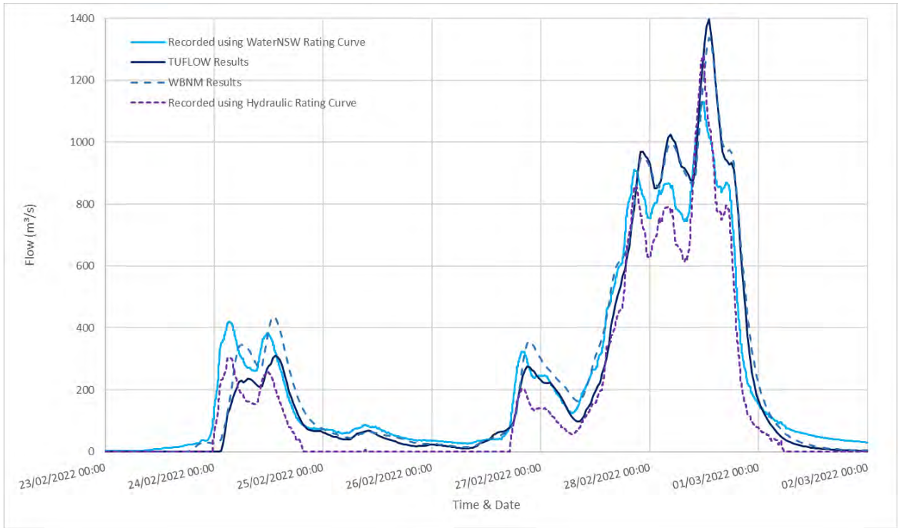
Diagram 76: 2022 Comparison of Flow at Palmers Road
