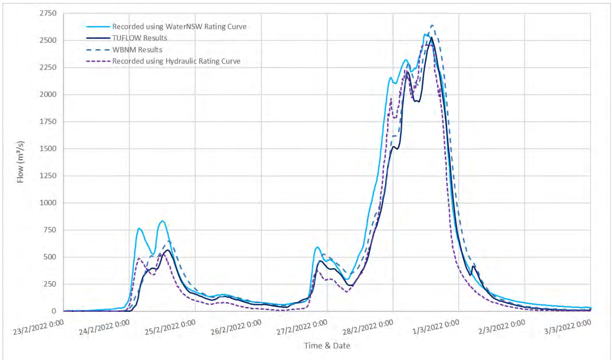
Diagram 77: 2022 Comparison of Flow at Uki
