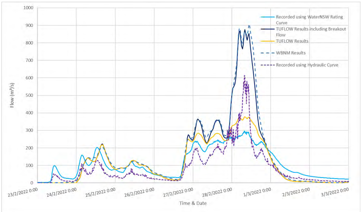
Diagram 79: 2022 Comparison of Flow at Boat Harbour
