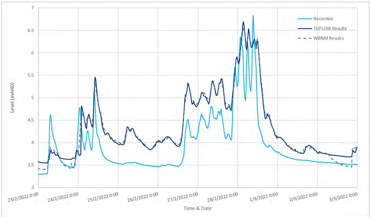
Diagram 84: 2022 Comparison of Water Level at Cobaki Creek
