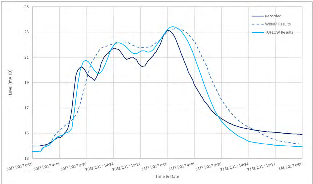
Diagram 66: 2017 Comparison of Water Level at Eungella
