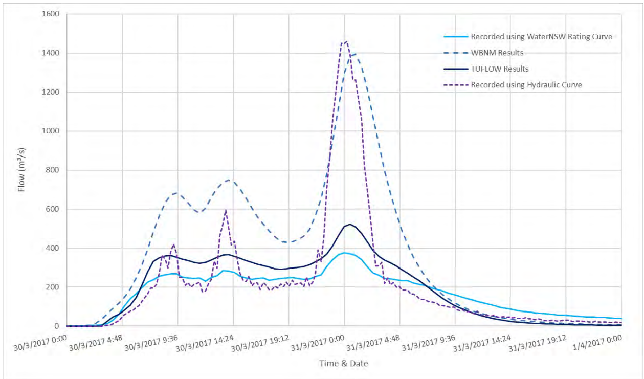
Diagram 62: 2017 Comparison of Flow at Boat Harbour
