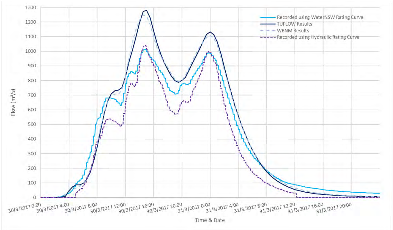
Diagram 59: 2017 Comparison of Flow at Palmers Road
