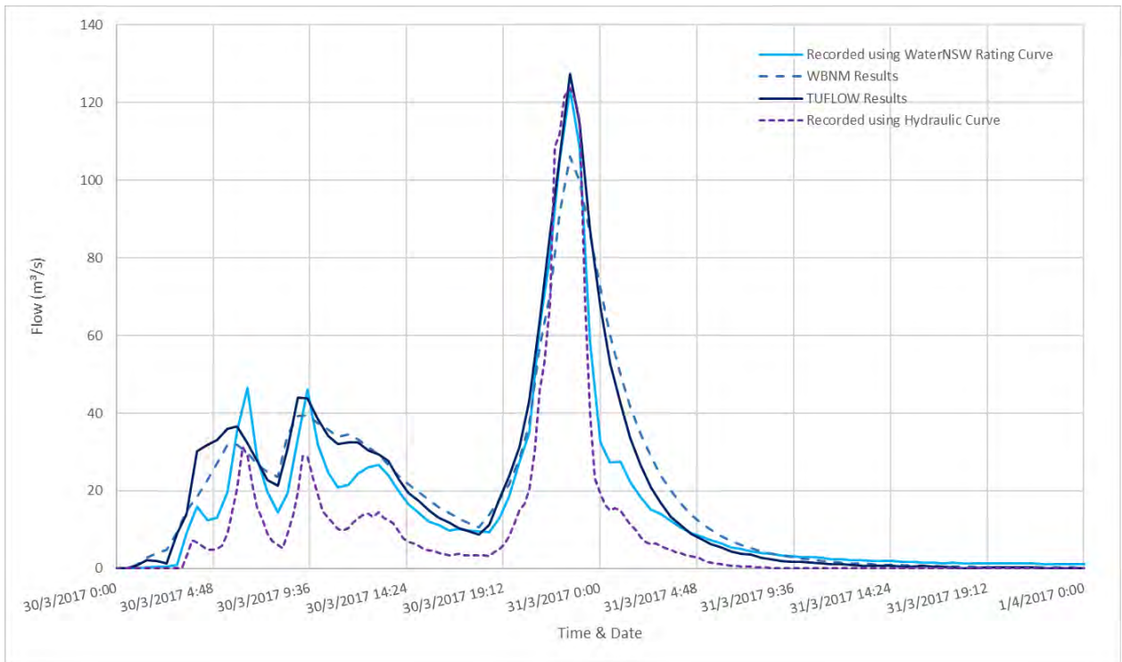
Diagram 63: 2017 Comparison of Flow at Cobaki Creek
