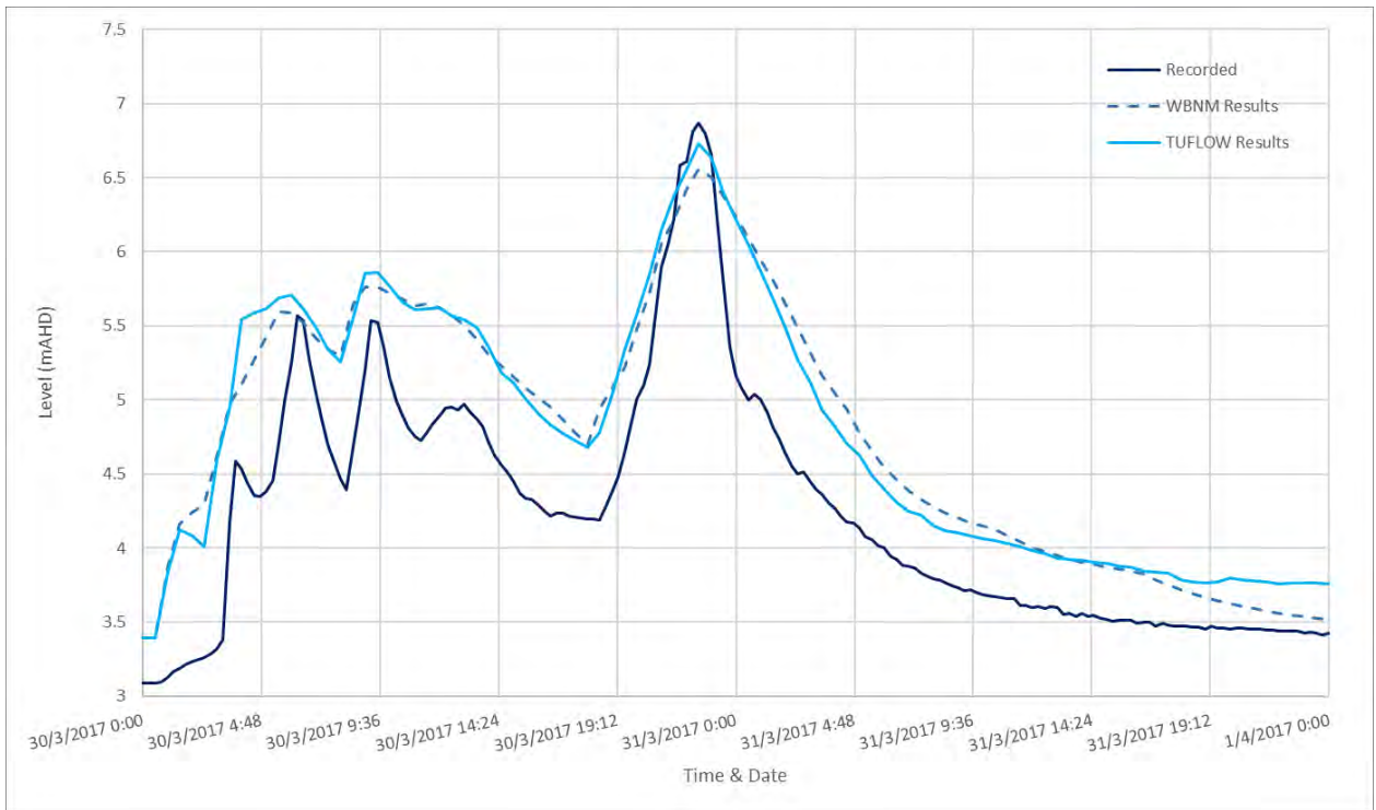
Diagram 68: 2017 Comparison of Water Level at Cobaki Creek
