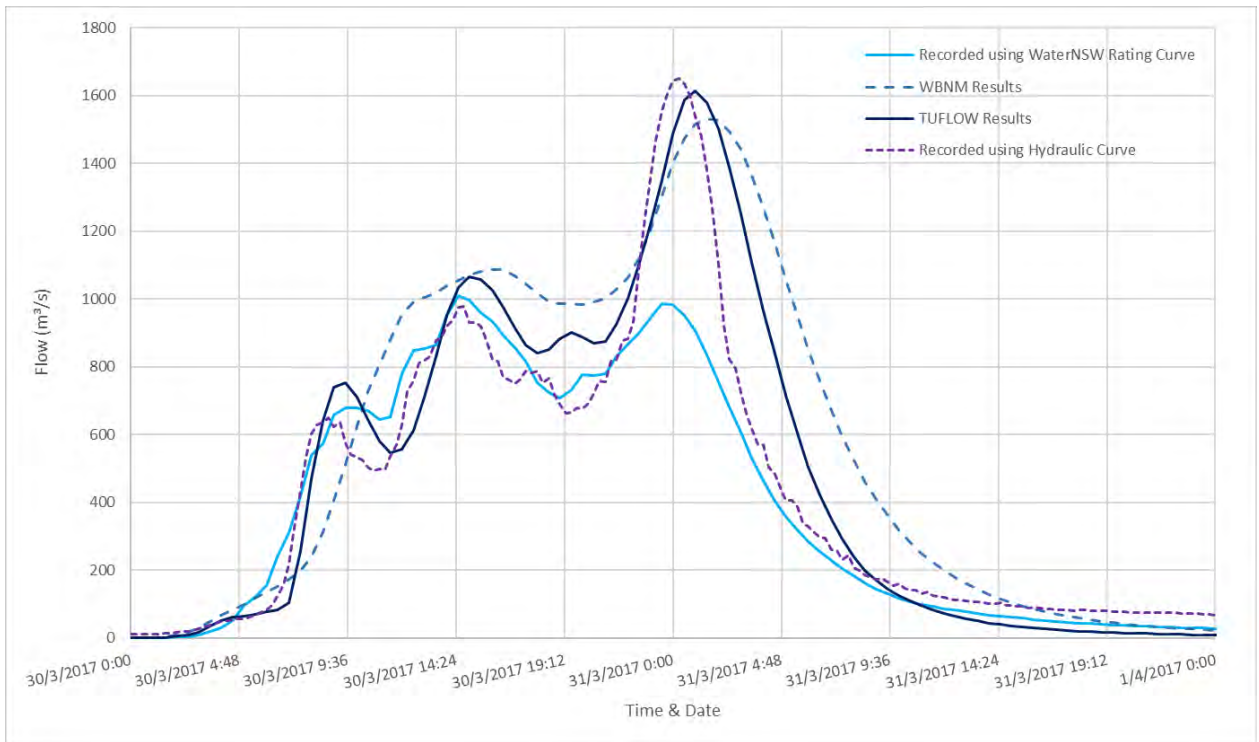
Diagram 61: 2017 Comparison of Flow at Eungella
