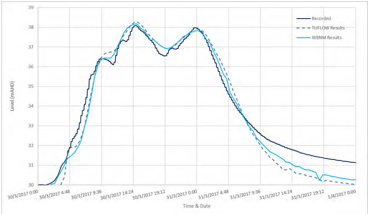
Diagram 64: 2017 Comparison of Water Level at Palmers Road
