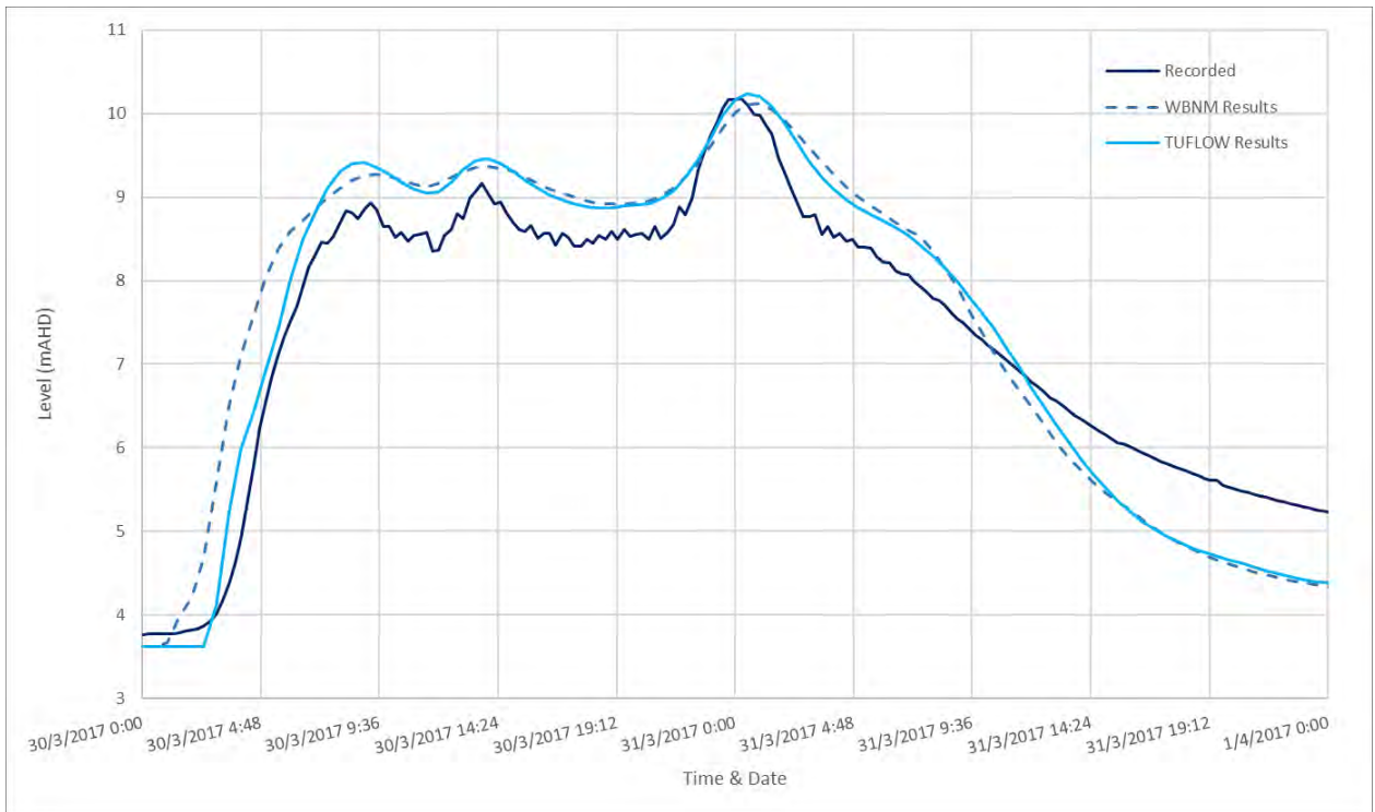
Diagram 67: 2017 Comparison of Water Level at Boat Harbour
