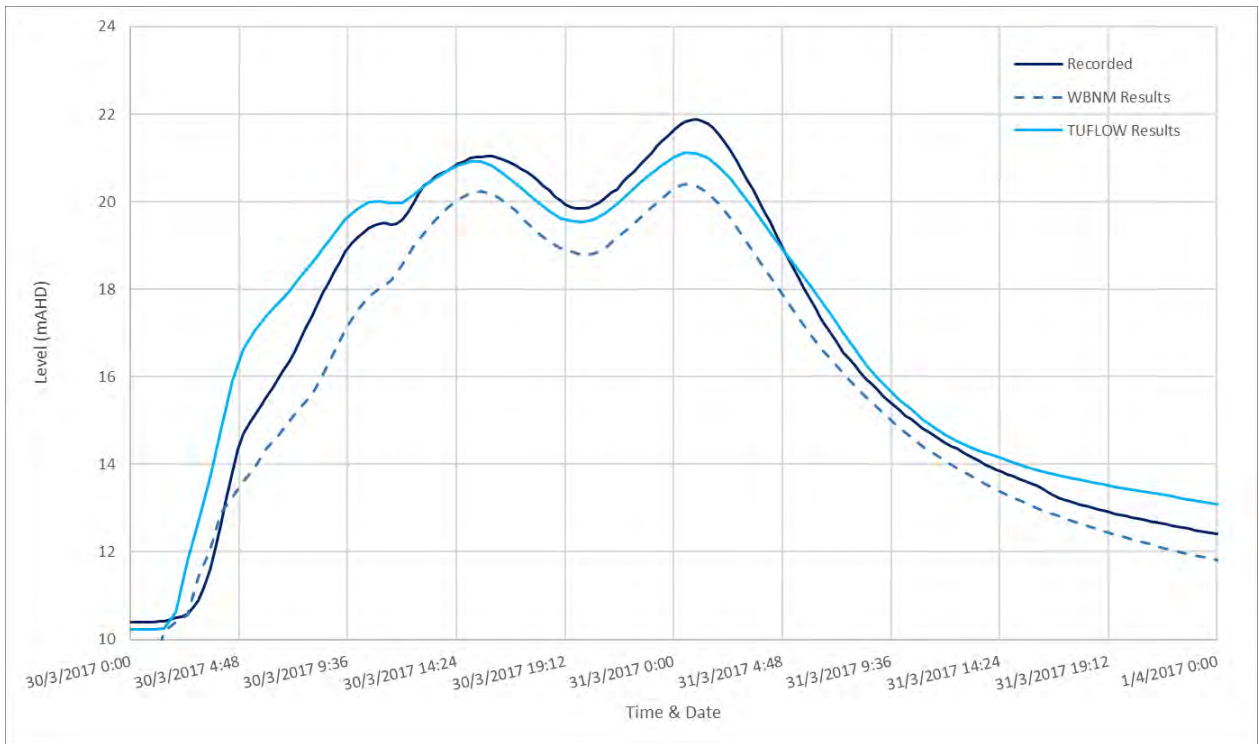
Diagram 65: 2017 Comparison of Water Level at Uki
