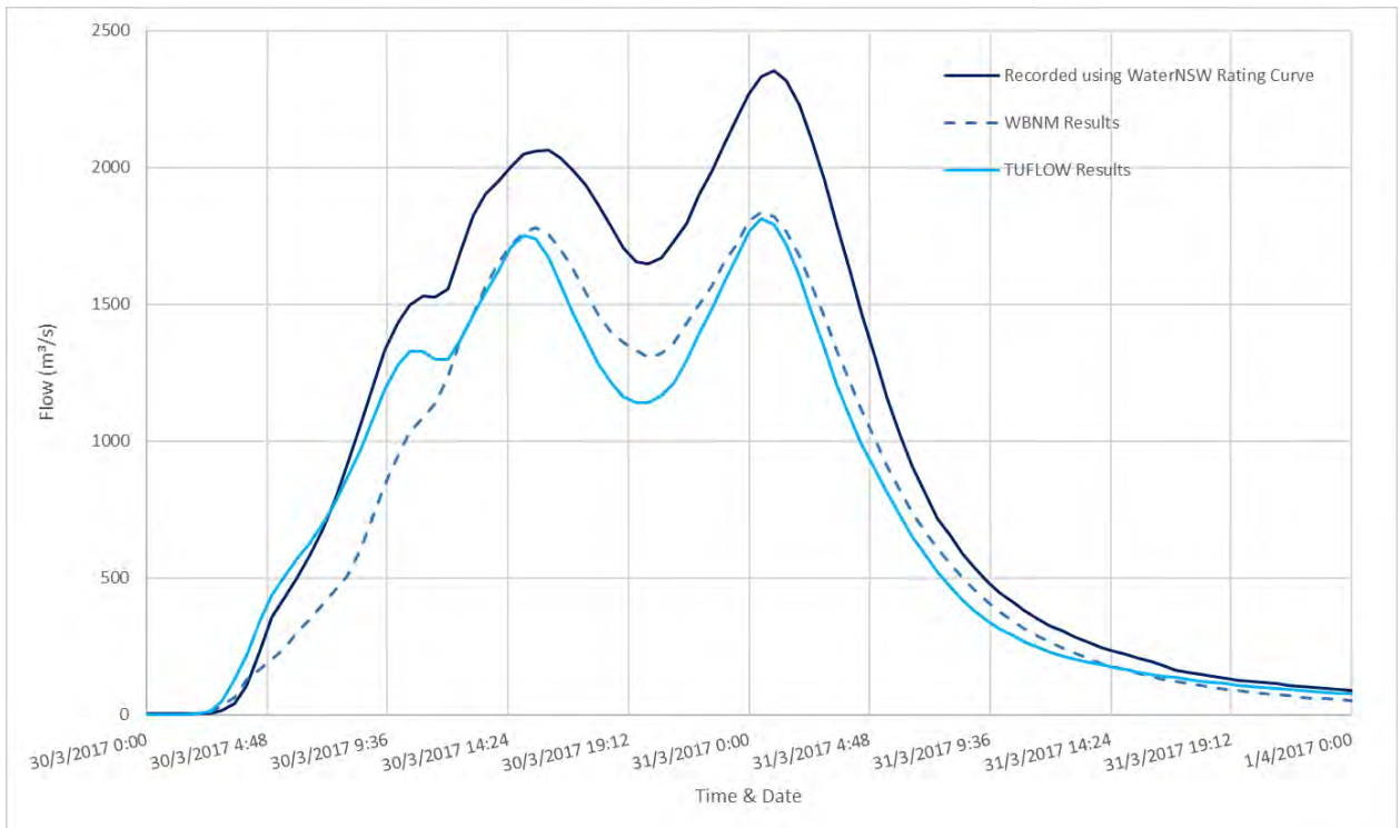
Diagram 60: 2017 Comparison of Flow at Uki
