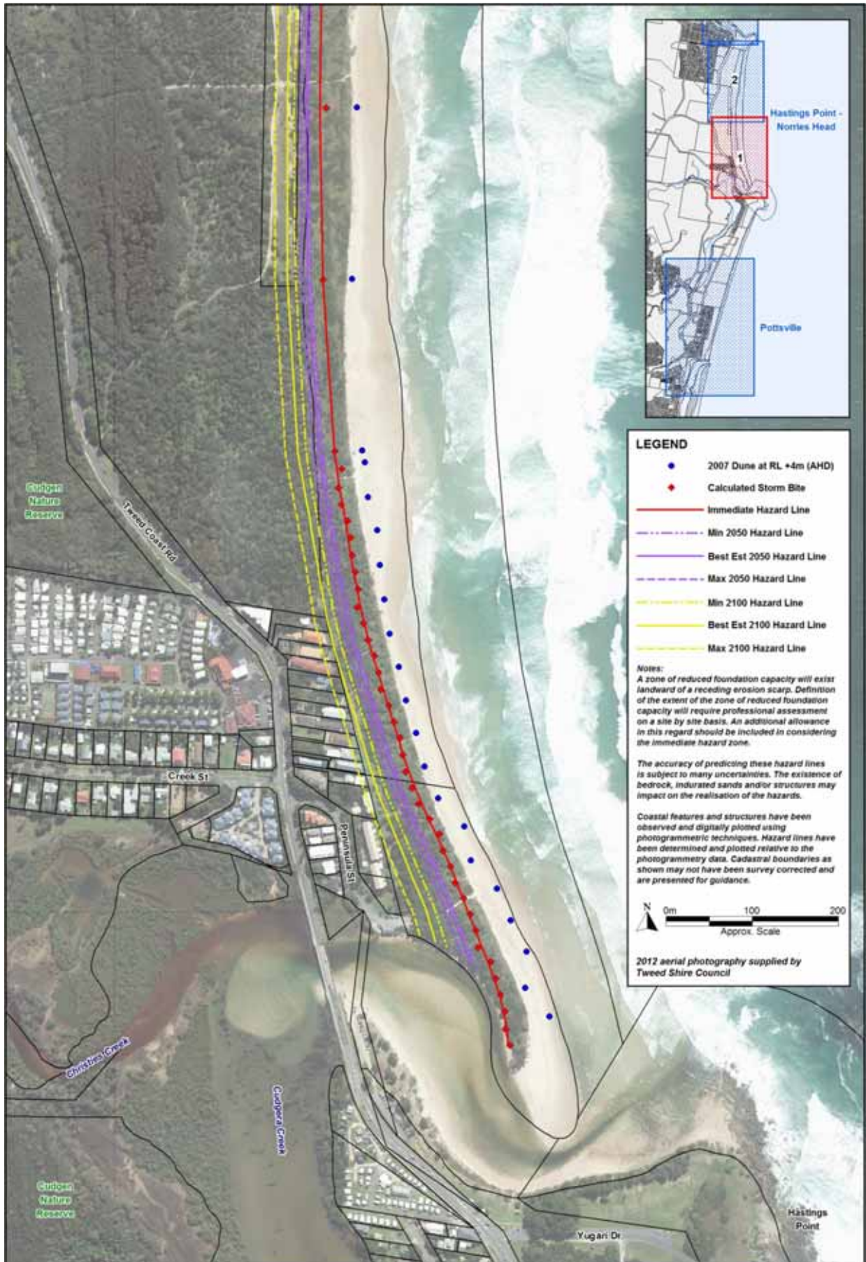
Figure 5-9 Erosion hazard extents: Hastings Point
