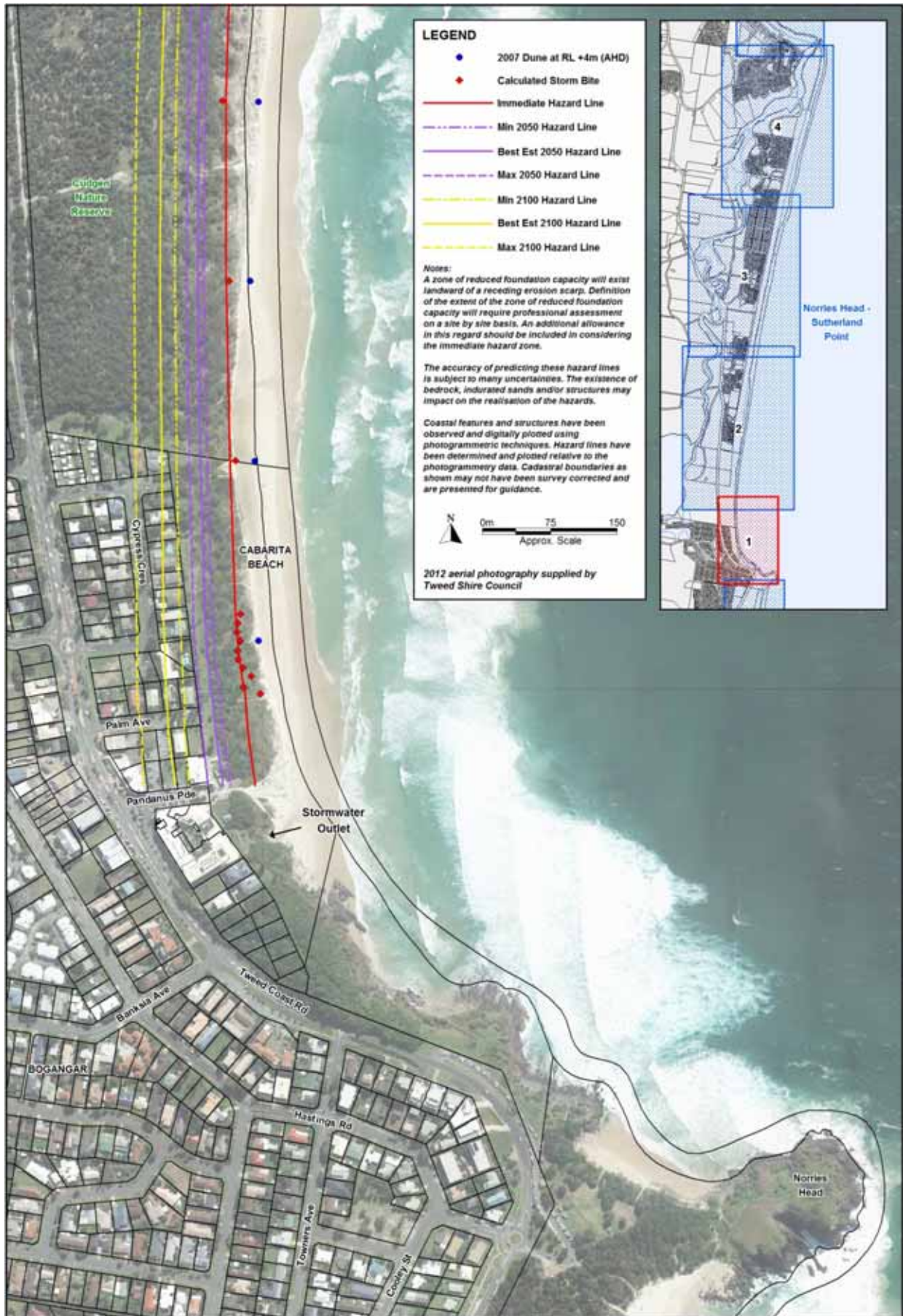
Figure 5-19 Erosion hazard extents for Cabarita Beach
