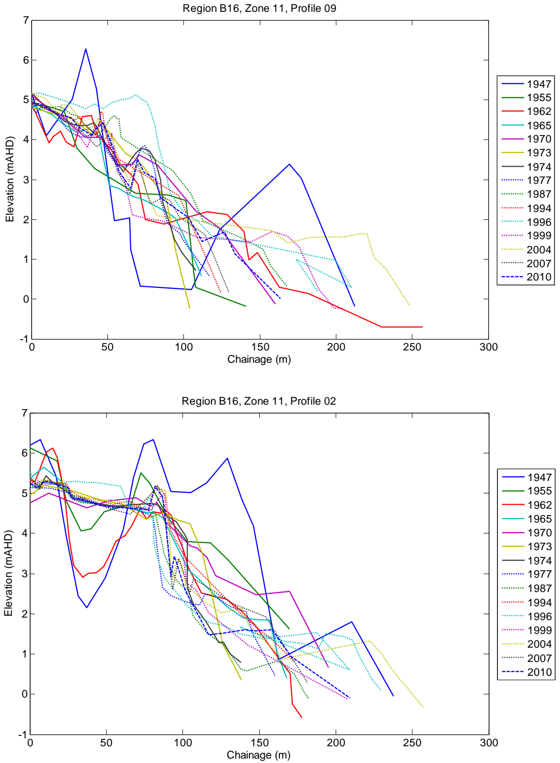
Figure A- 9 Kingscliff Photogrammetry Profiles: Zone 11 (Surf Club) Locations shown in Figure 4-6
