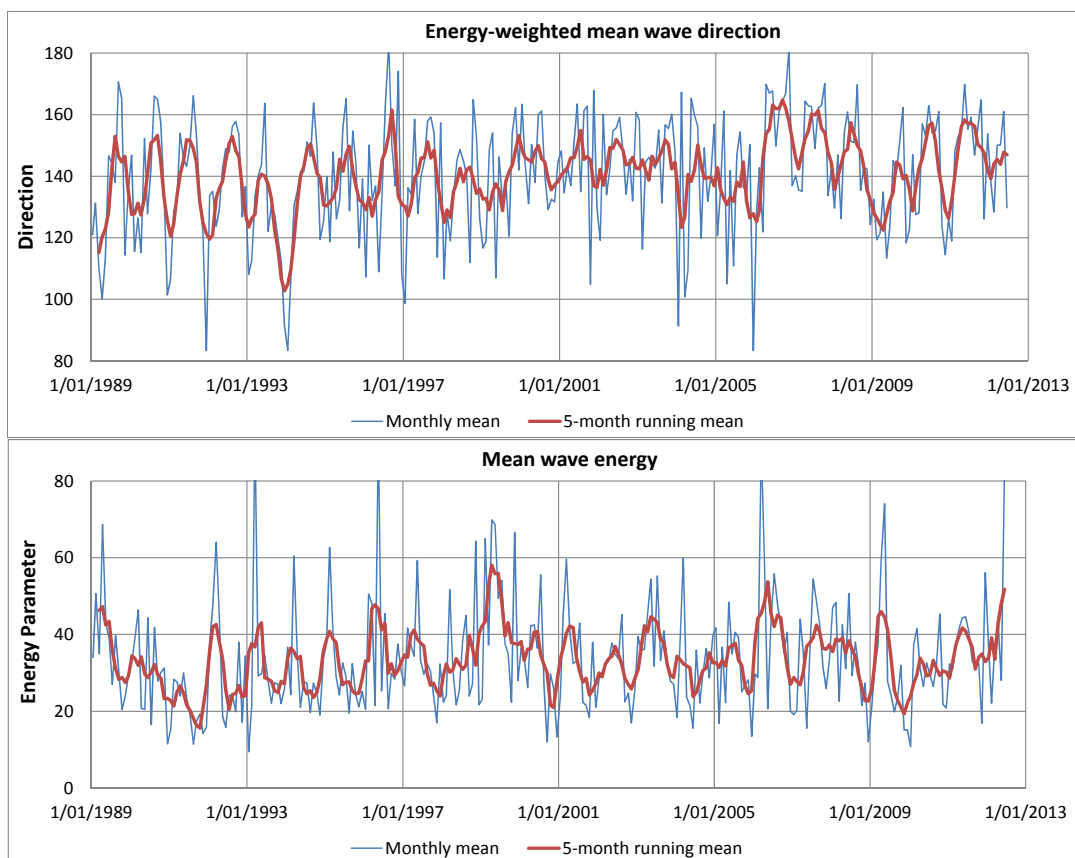
Figure 2-18 Monthly mean wave direction (top) and energy factor (bottom) since 1997
