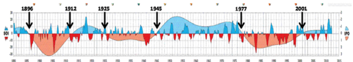
Figure 2-17 Correlated ENSO and IPO patterns since 1890
