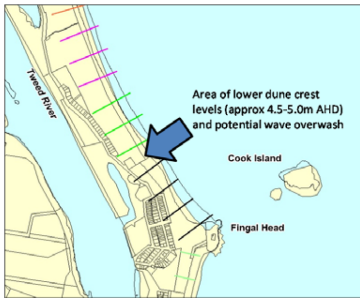
Figure 5-29 Zone of limited potential wave overshoot – Letitia Spit
