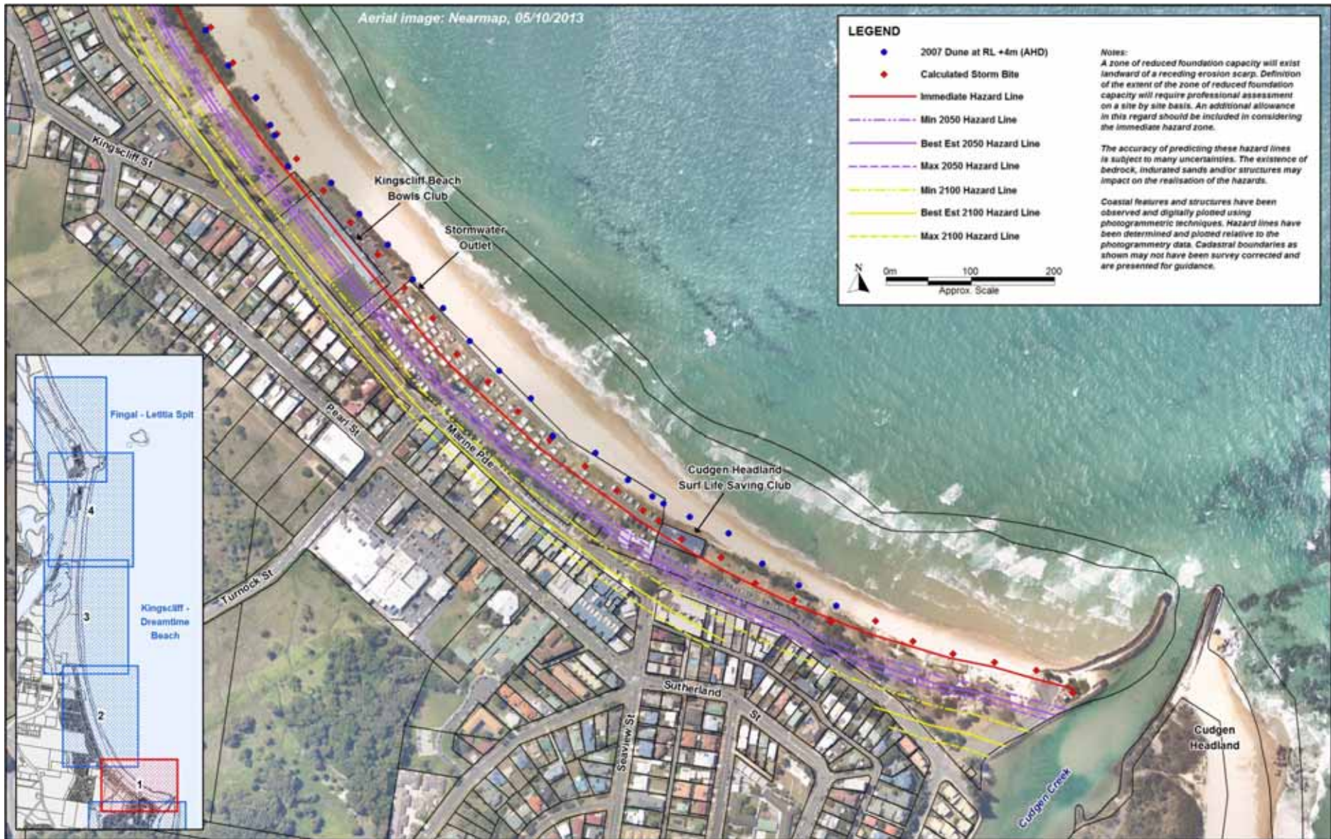
Figure 4-8 Erosion hazard zones: Kingscliff
