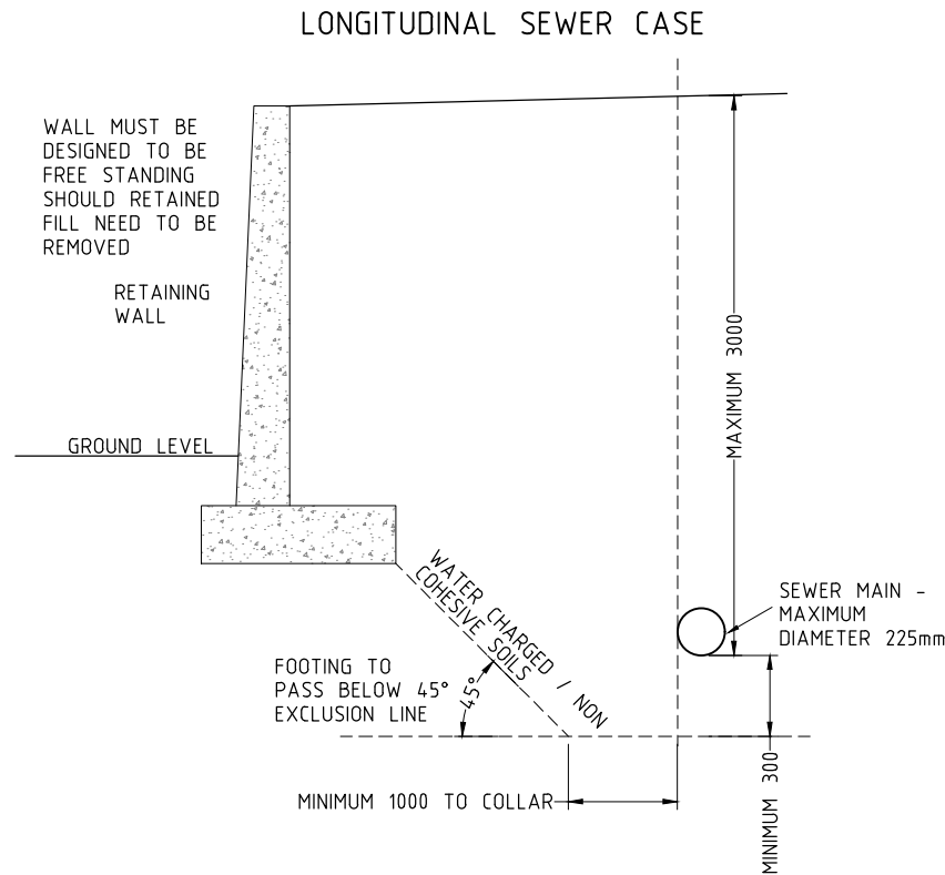
REFER TO DRAWING S.D.281 FOOTING CASE 2. WATER CHARGED / NON COHESIVE SOILS
