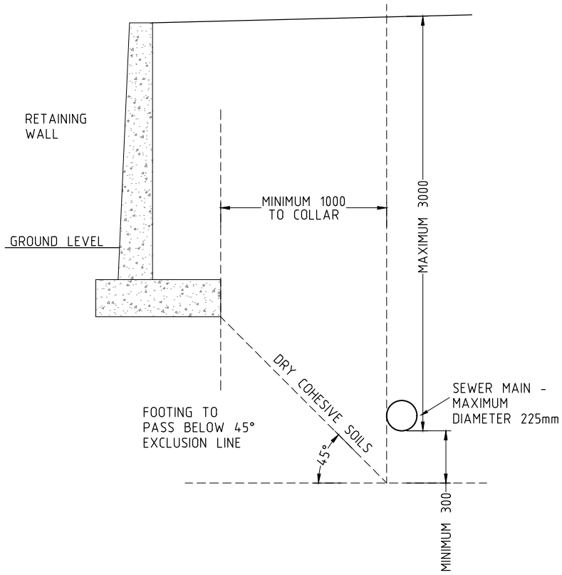
REFER TO DRAWING S.D.281 FOOTING CASE 1. DRY COHESIVE SOILS
