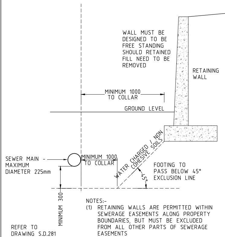
REFER TO DRAWING S.D.281 FOOTING CASE 2. WATER CHARGED / NON COHESIVE SOILS
