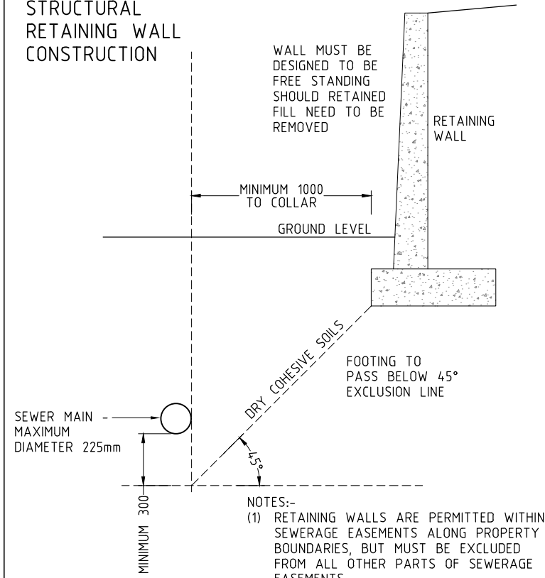
REFER TO DRAWING S.D.281 FOOTING CASE 1. DRY COHESIVE SOILS
