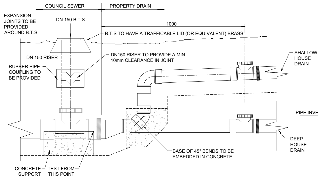
ELEVATION STANDARD HOUSE DRAIN CONNECTION TO SEWER FOR DRIVEWAYS
