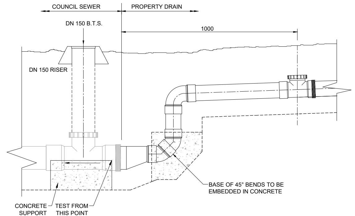
ELEVATION STANDARD DEEP HOUSE DRAIN CONNECTION TO SEWER
