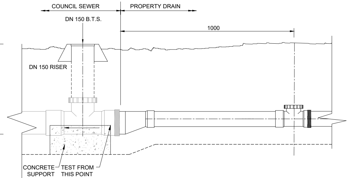
ELEVATION STANDARD SHALLOW HOUSE DRAIN CONNECTION TO SEWER
