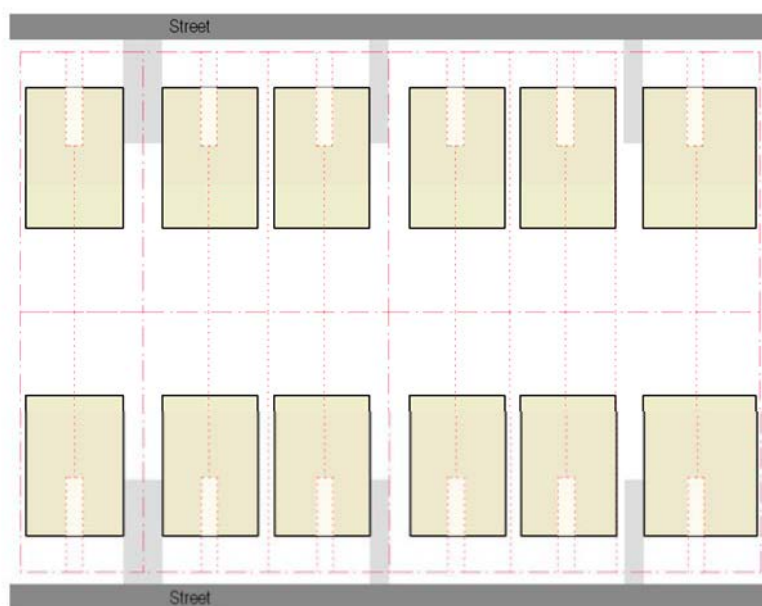
Illustrative block layout for the Small Residential Flat Building
