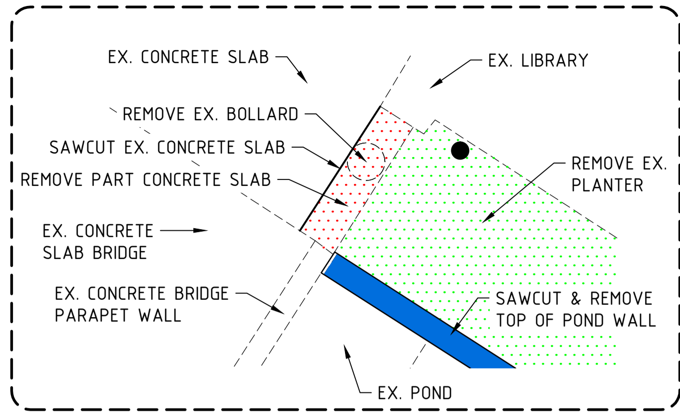
INSET PLAN SCALE 1:20
