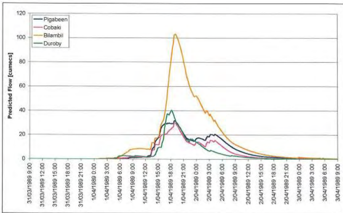
Figure 4-34 Modelled Hydrographs, Lower Tweed, April 1989
