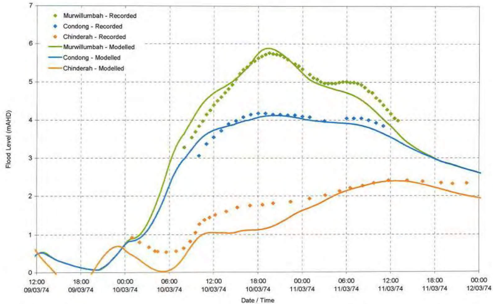
Figure 4-10 Recorded and Modelled Flood Levels, March 1974
