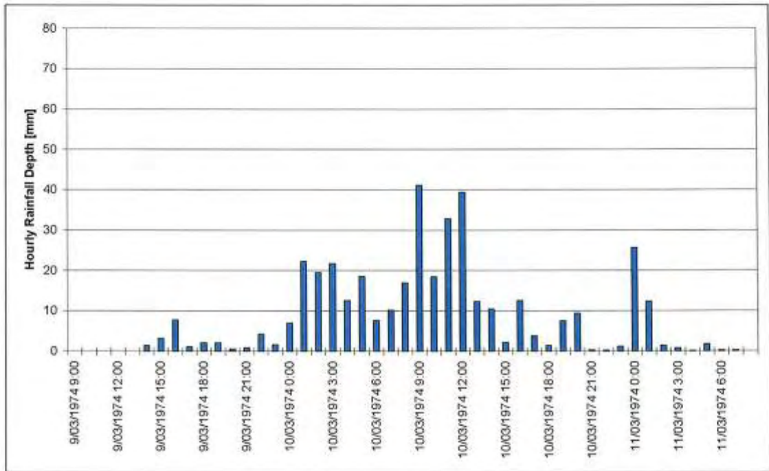
Figure 4-1 Tyalgum (Pumpenbil Rd) Pluviometer, March 1974
