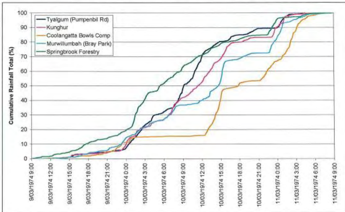
Figure 4-6 Cumulative Rainfall, March 1974
