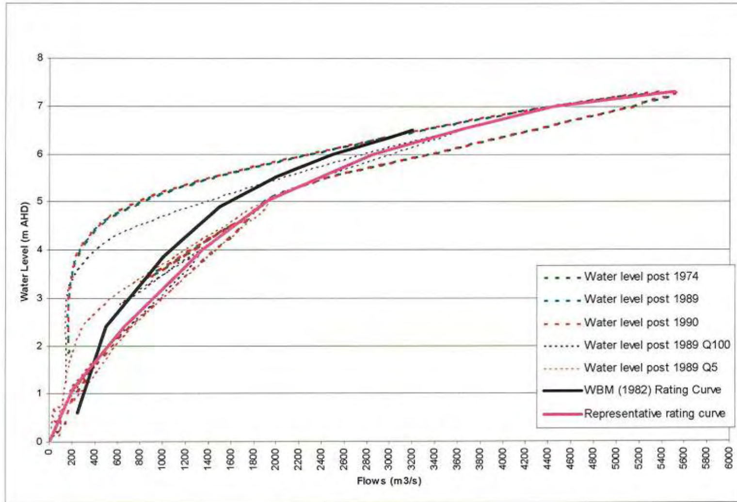
Figure A-1 Rating Curves
