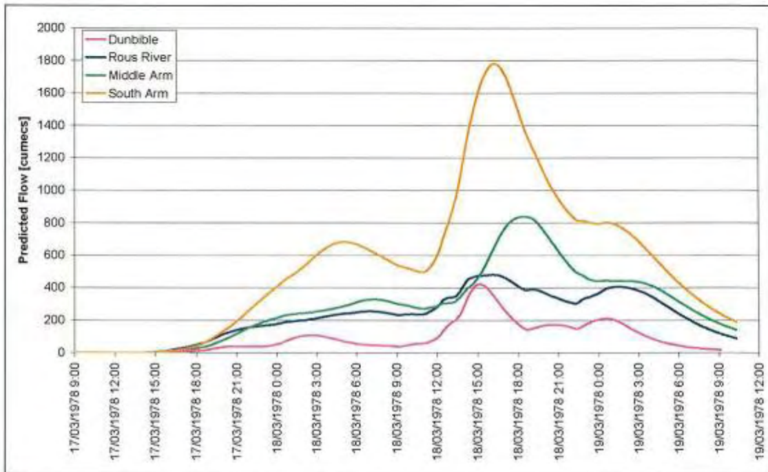
Figure 4-22 Modelled Hydrographs, Upper Tweed, March 1978
