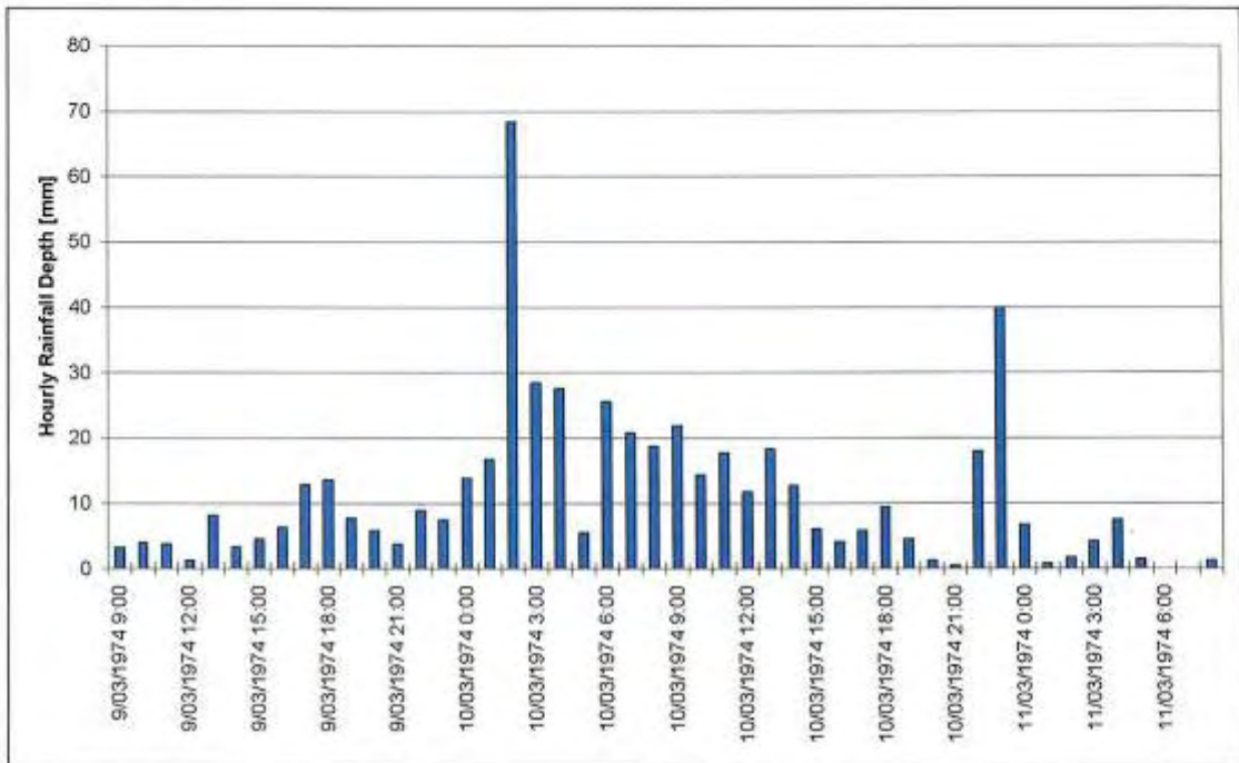
Figure 4-5 Springbrook Forestry Pluviometer, March 1974
