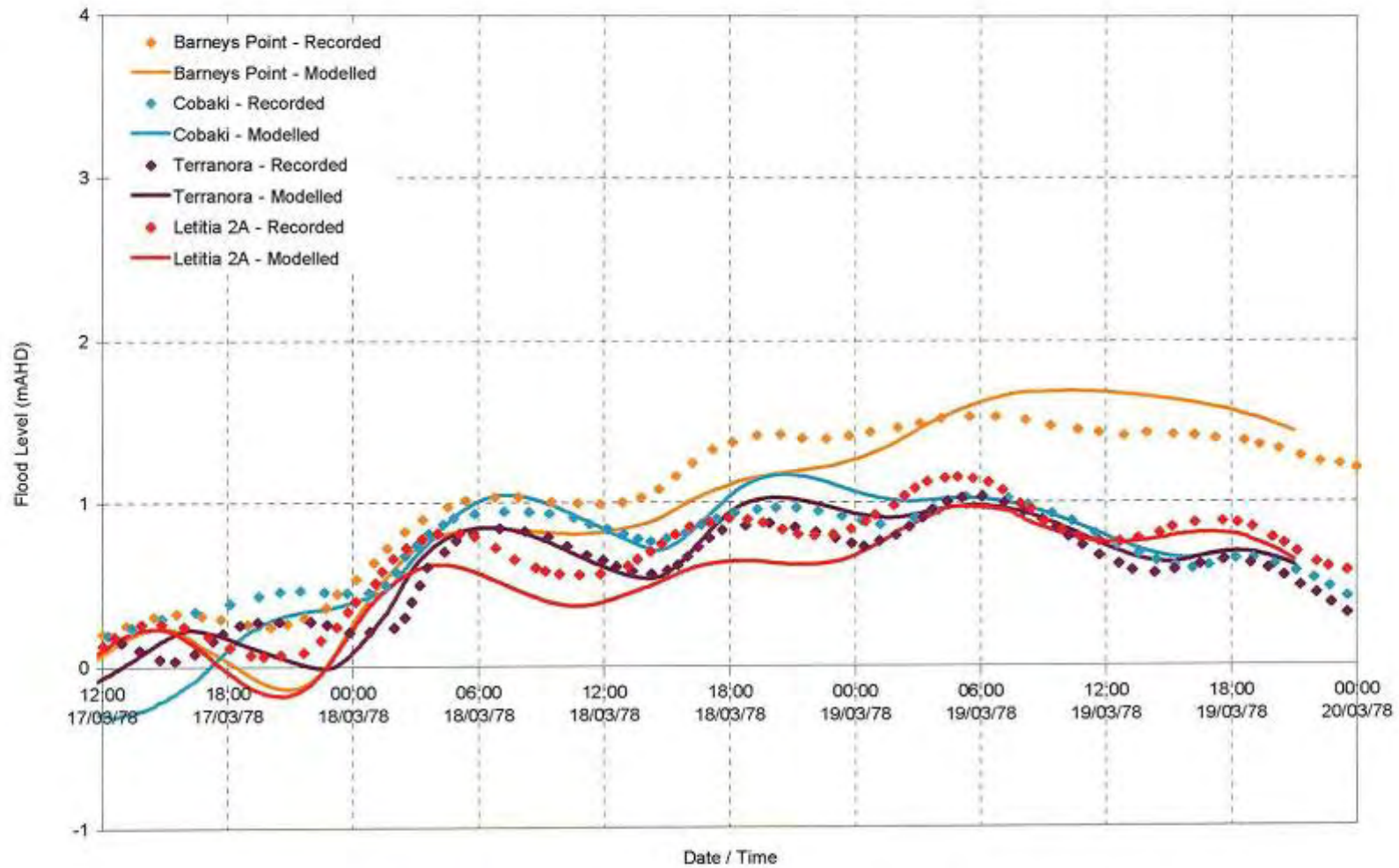
Figure 4-24 Recorded and Modelled Flood Levels, Lower Tweed, March 1978
