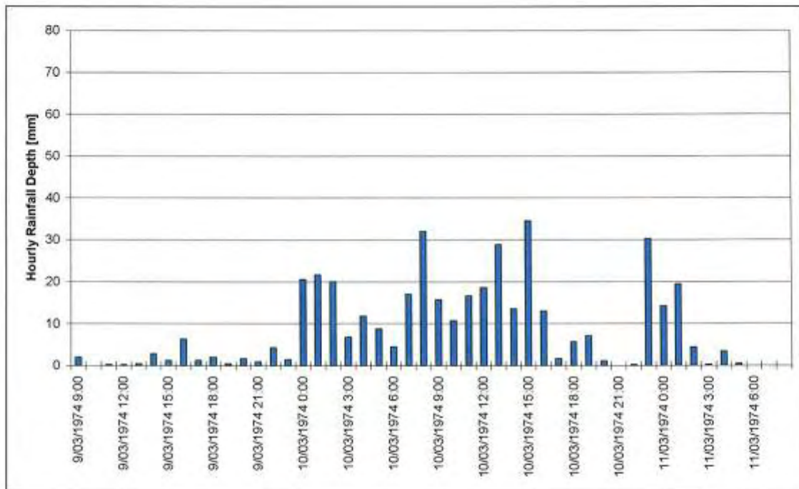
Figure 4-2 Kunghur Pluviometer, March 1974
