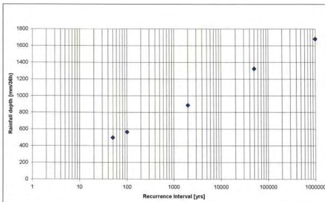
Figure 5-2 Design Rainfall Depths, 36 Hour Storm
