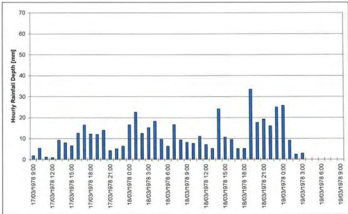
Figure 4-15 Springbrook Forestry Pluviometer, March 1978
