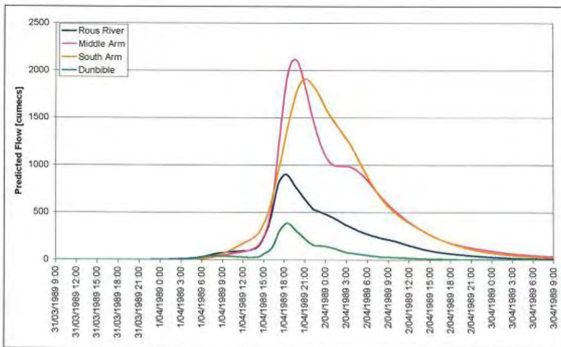
Figure 4-35 Modelled Hydrographs, Upper Tweed, April 1989
