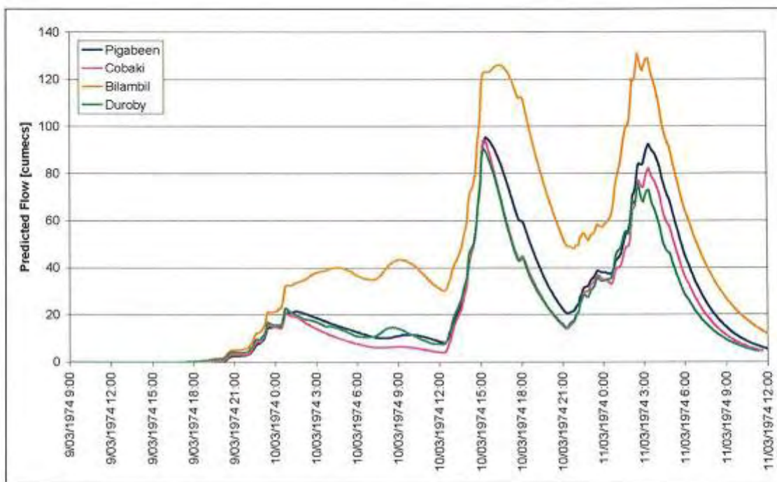
Figure 4-8 Modelled Hydrographs, Lower Tweed, March 1974
