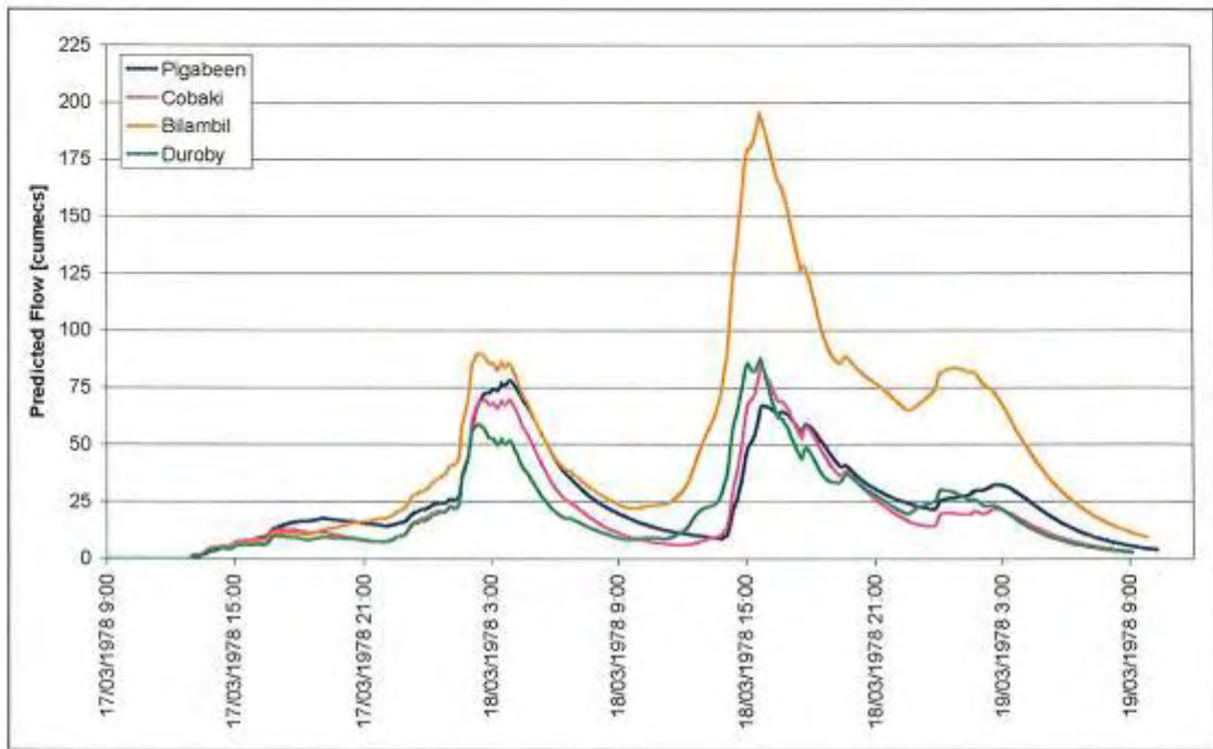
Figure 4-21 Modelled Hydrographs, Lower Tweed, March 1978
