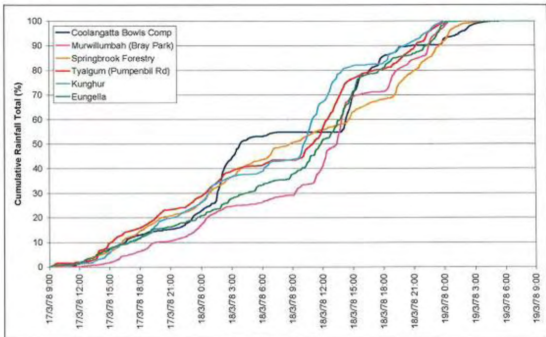
Figure 4-19 Cumulative Totals, March 1978
