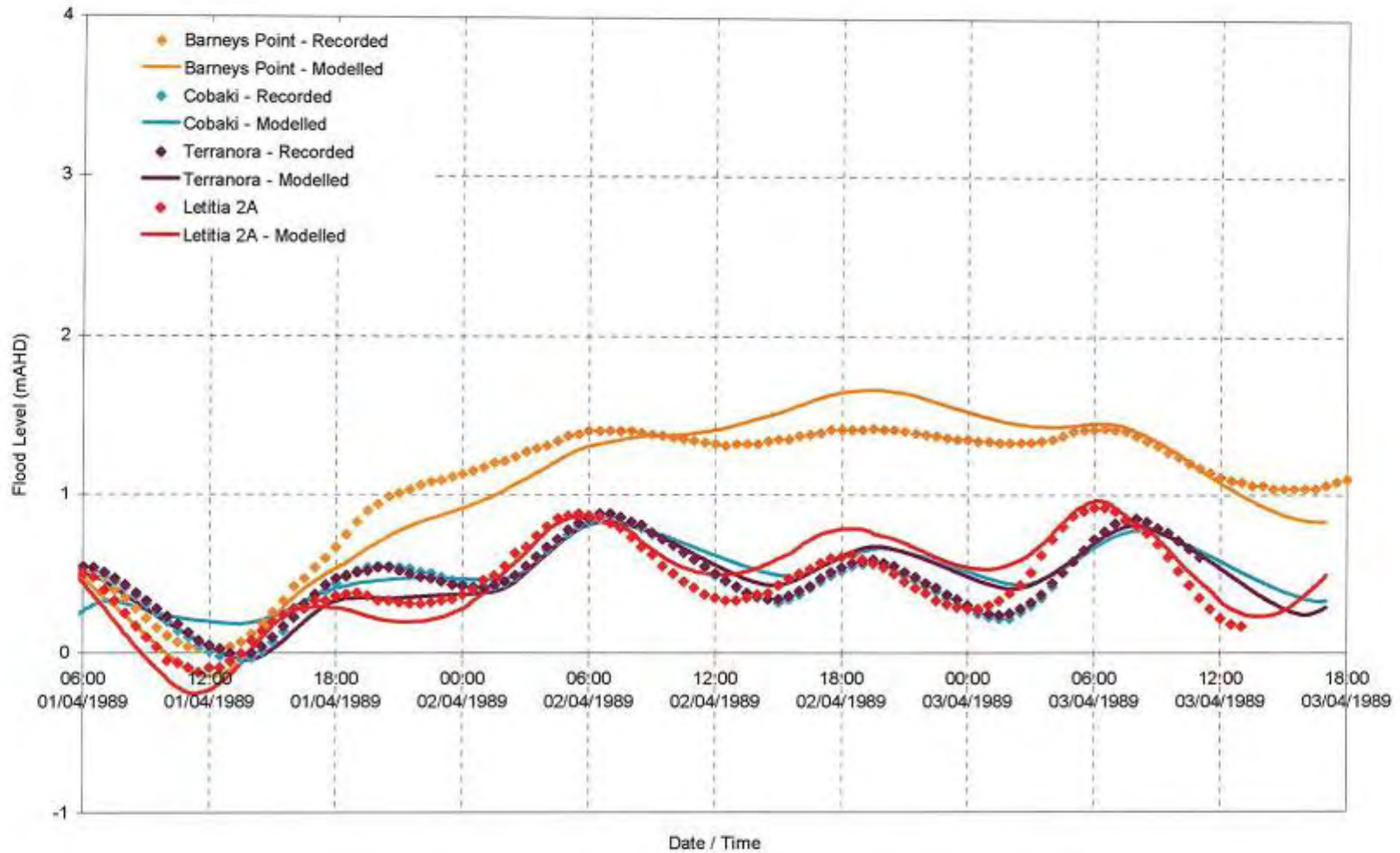
Figure 4-37 Recorded and Modelled Flood Levels, Lower Tweed, April 1989
