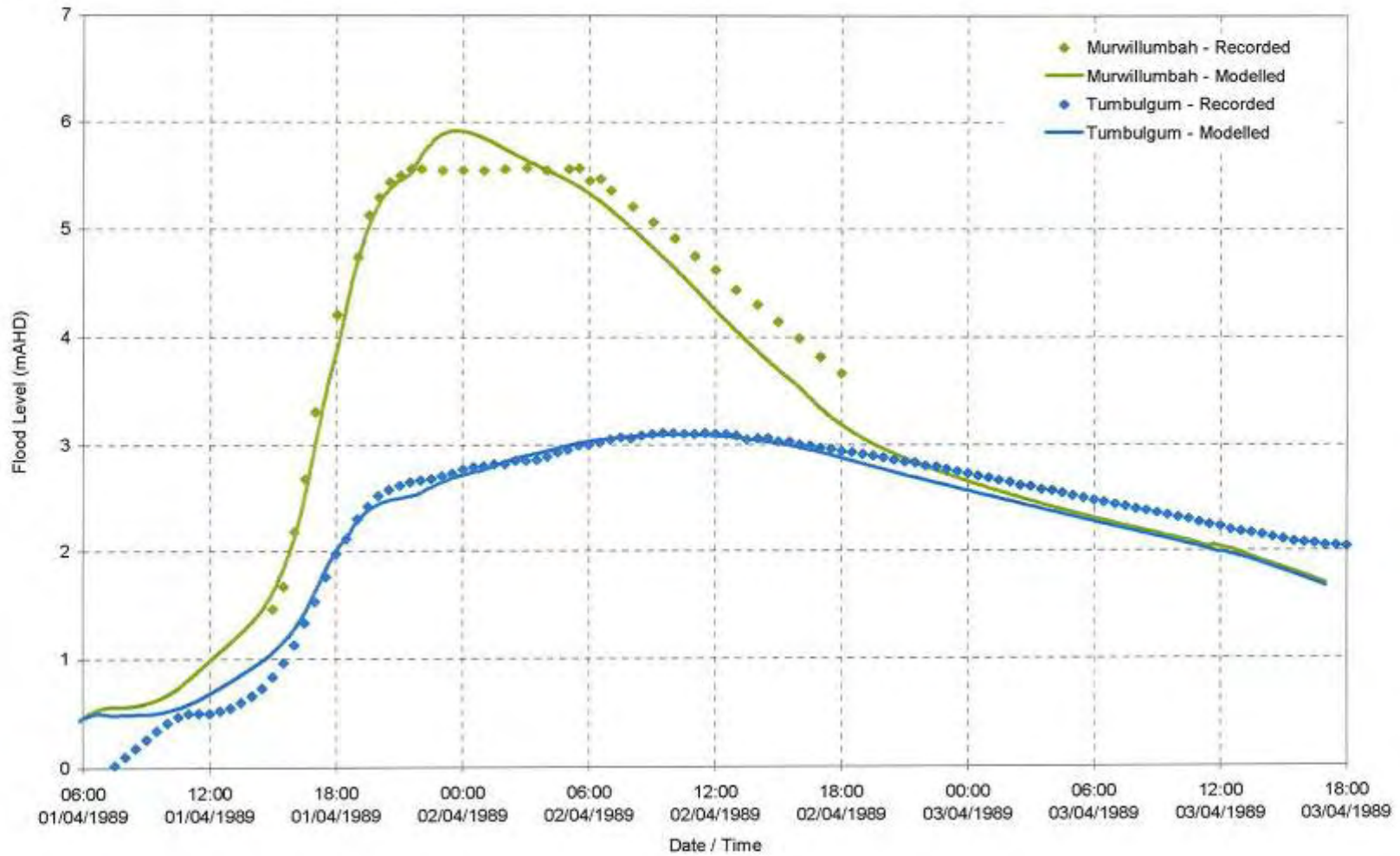
Figure 4-36 Recorded and Modelled Flood Levels, Upper Tweed, April 1989
