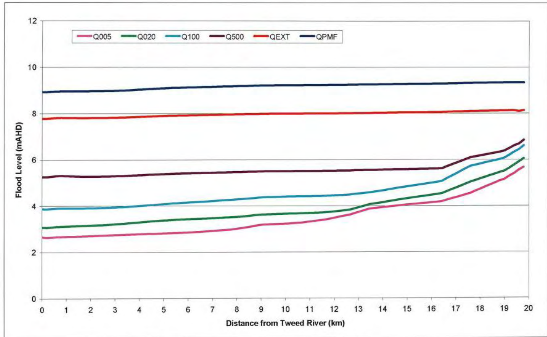
Figure 6-4 Design Flood Profile, Rous River
