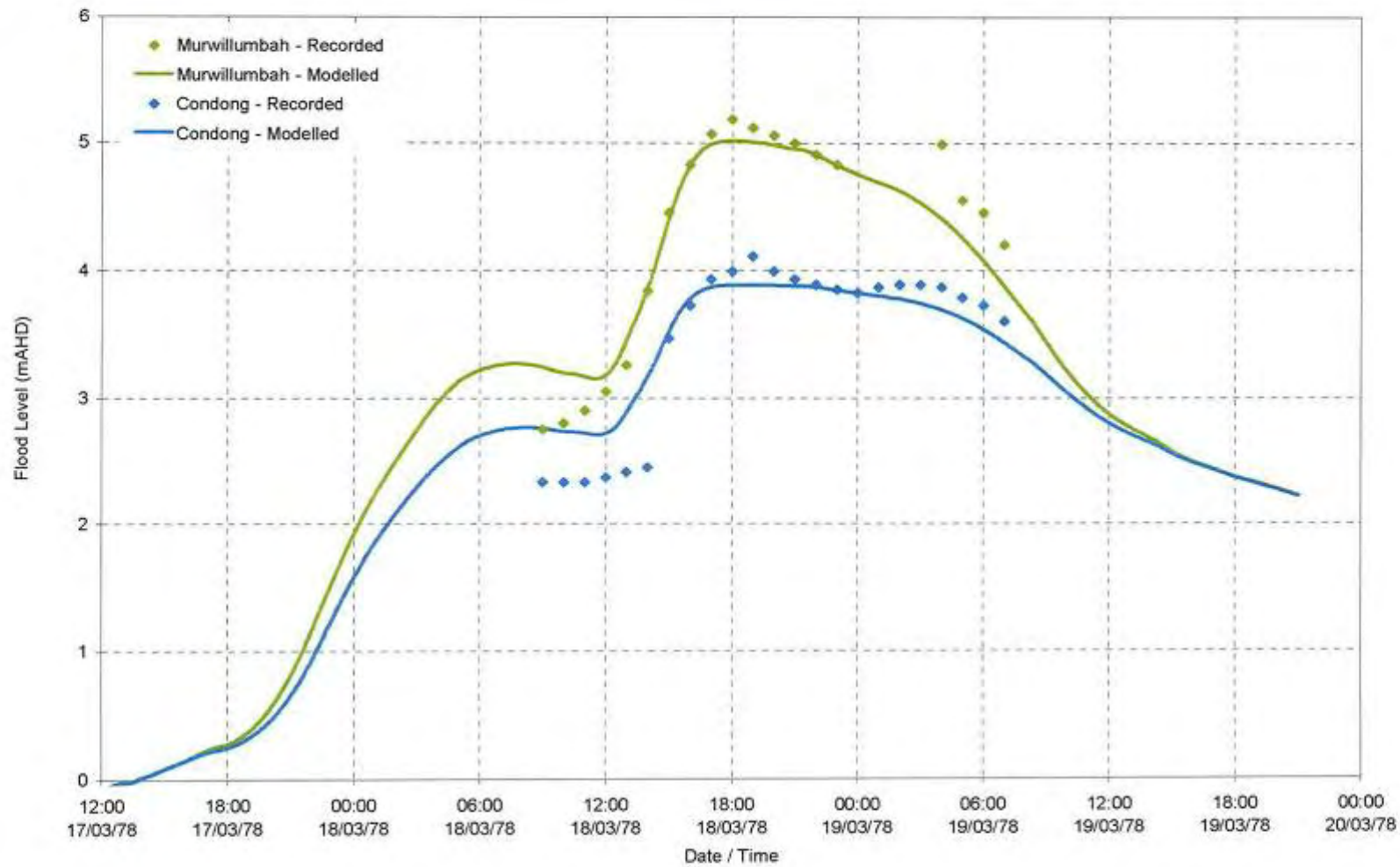
Figure 4-23 Recorded and Modelled Flood Levels, Upper Tweed, March 1978
