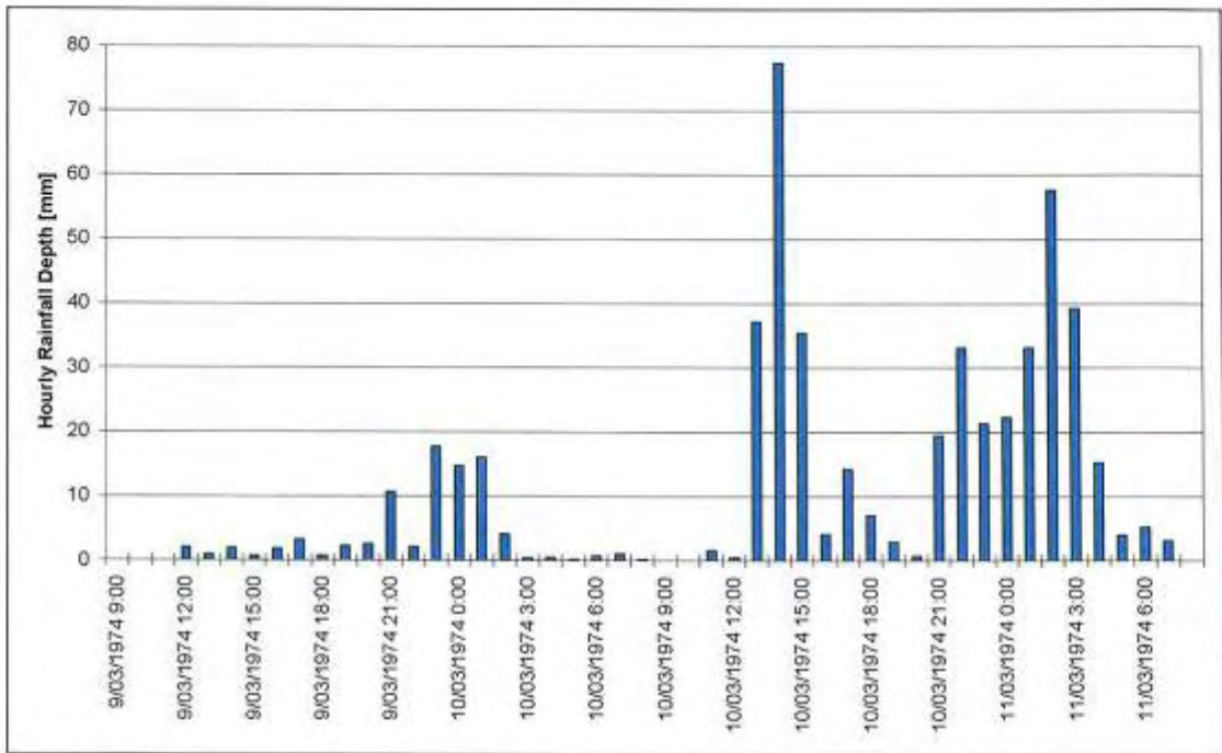
Figure 4-3 Coolangatta Bows Comp Pluviometer, March 1974
