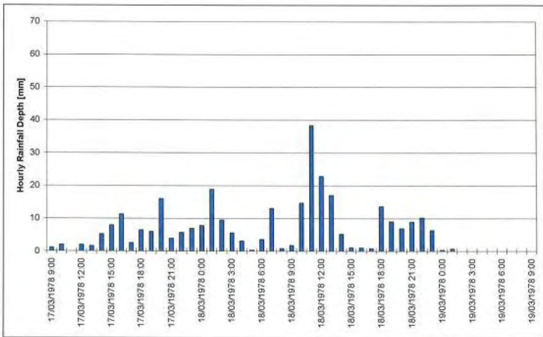
Figure 4-17 Kunghur Pluviometer, March 1978
