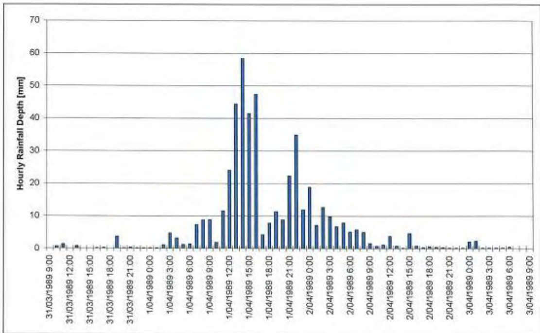
Figure 4-25 Tyalgum (Pumpenbil Rd) Pluviometer, April 1989
