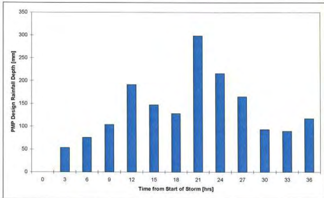
Figure 5-3 PMP Temporal Distribution, 36 Hour Storm
