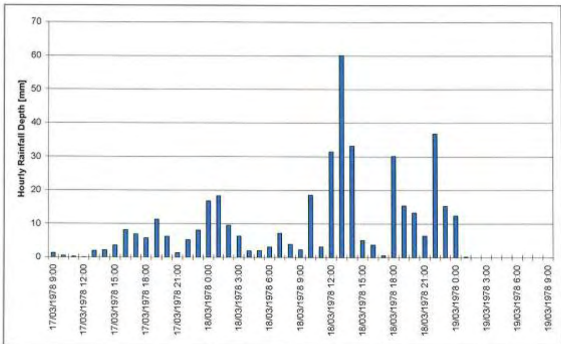
Figure 4-14 Murwillumbah (Bray Park) Pluviometer, March 1978
