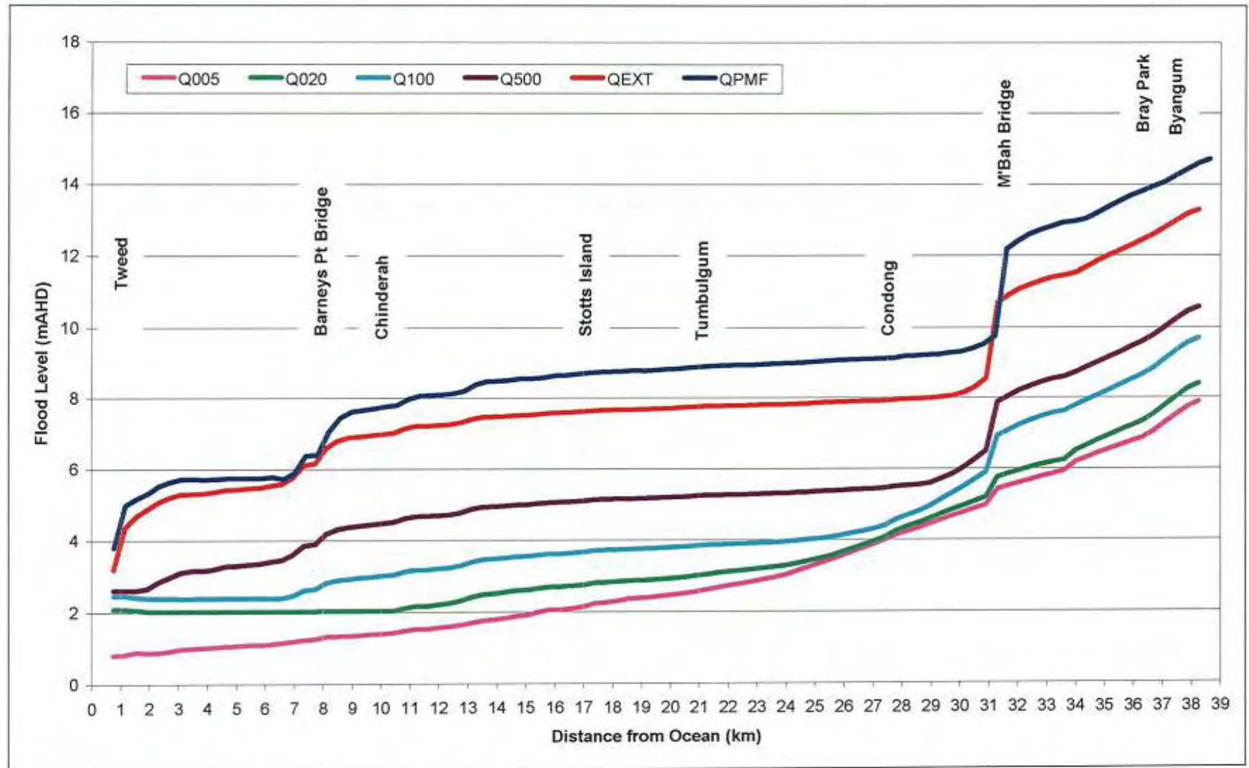
Figure 6-3 Design Flood Profile, Tweed River
