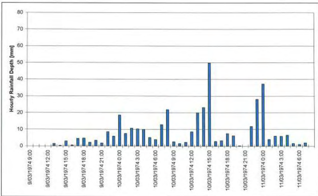
Figure 4-4 Murwillumbah (Bray Park) Pluviometer, March 1974
