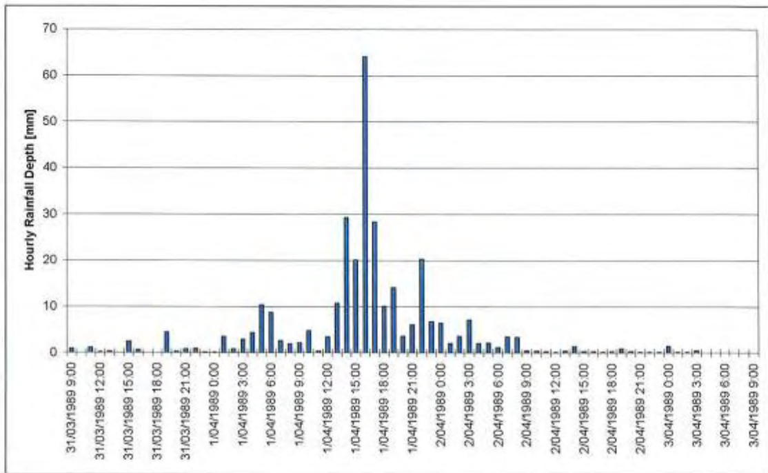
Figure 4-29 Murwillumbah (Bray Park) Pluviometer, April 1989
