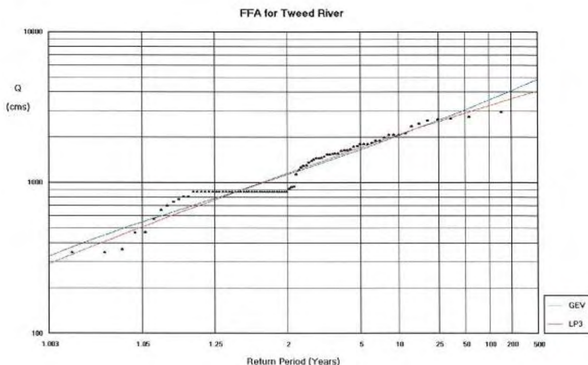
Figure A-1 Flood Frequency Analysis results
