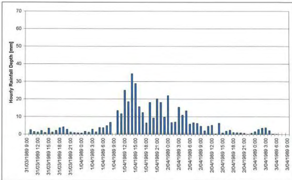
Figure 4-30 Springbrook Forestry Pluviometer, April 1989
