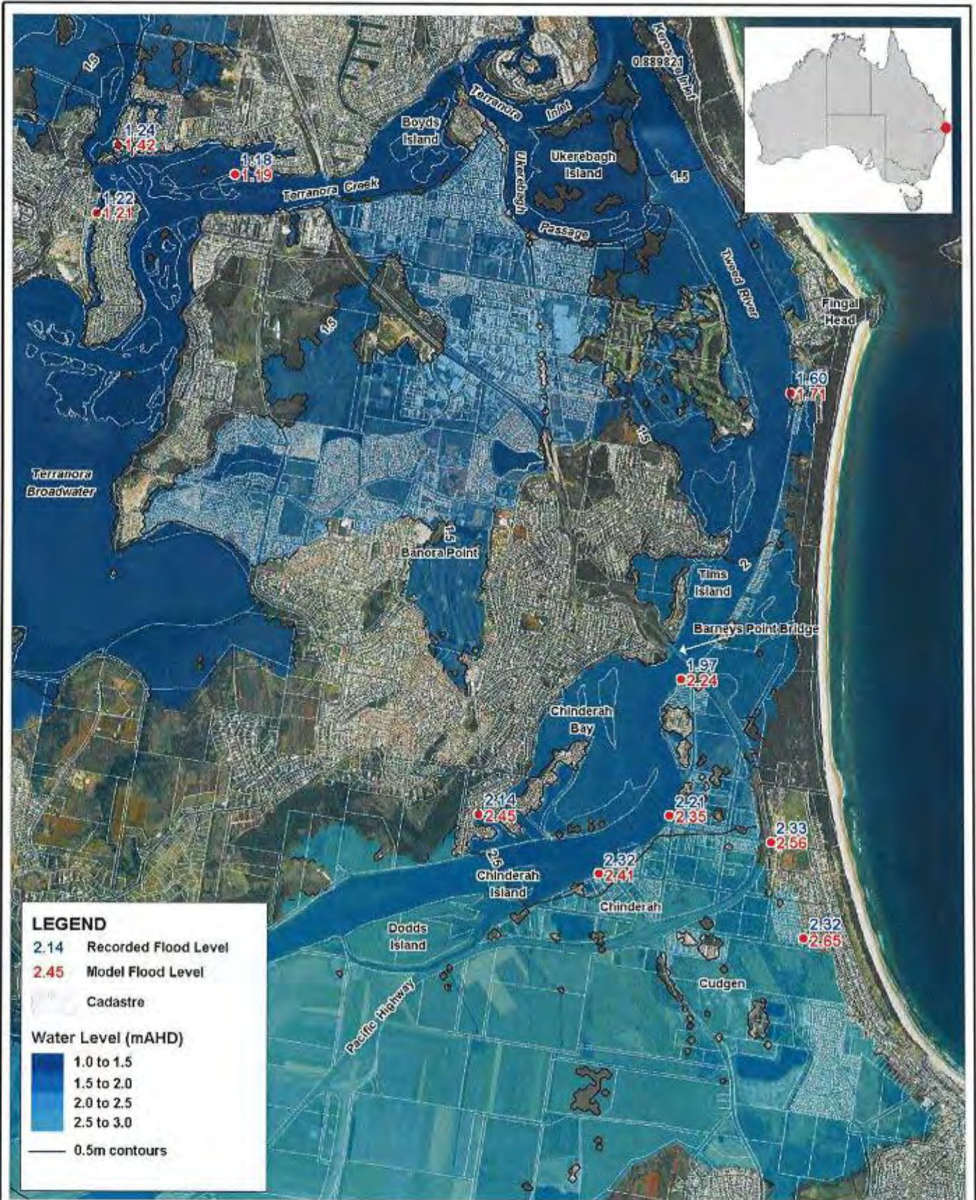
Title: Recorded and modelled Flood Levels Chinderah, March 1974
