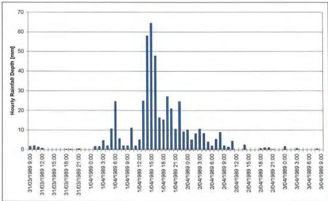
Figure 4-31 Eungella Pluviometer, April 1989
