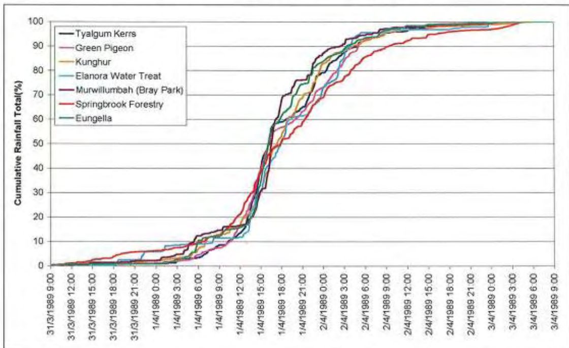
Figure 4-32 Cumulative Totals, April 1989
