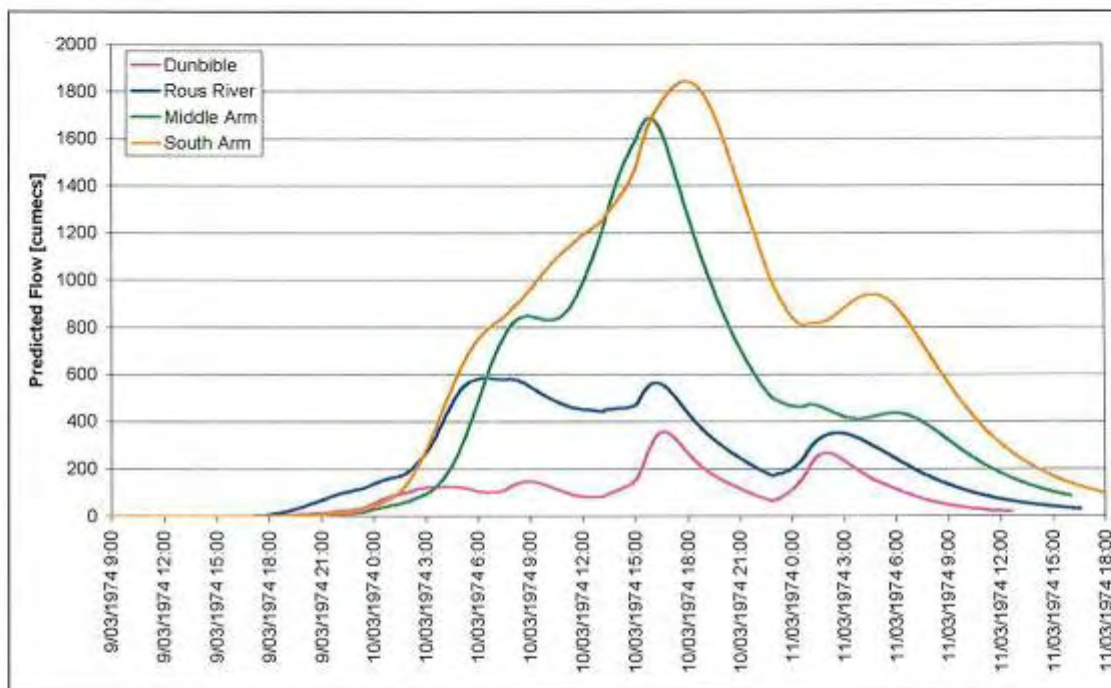
Figure 4-9 Modelled Hydrographs, Upper Tweed, March 1974
