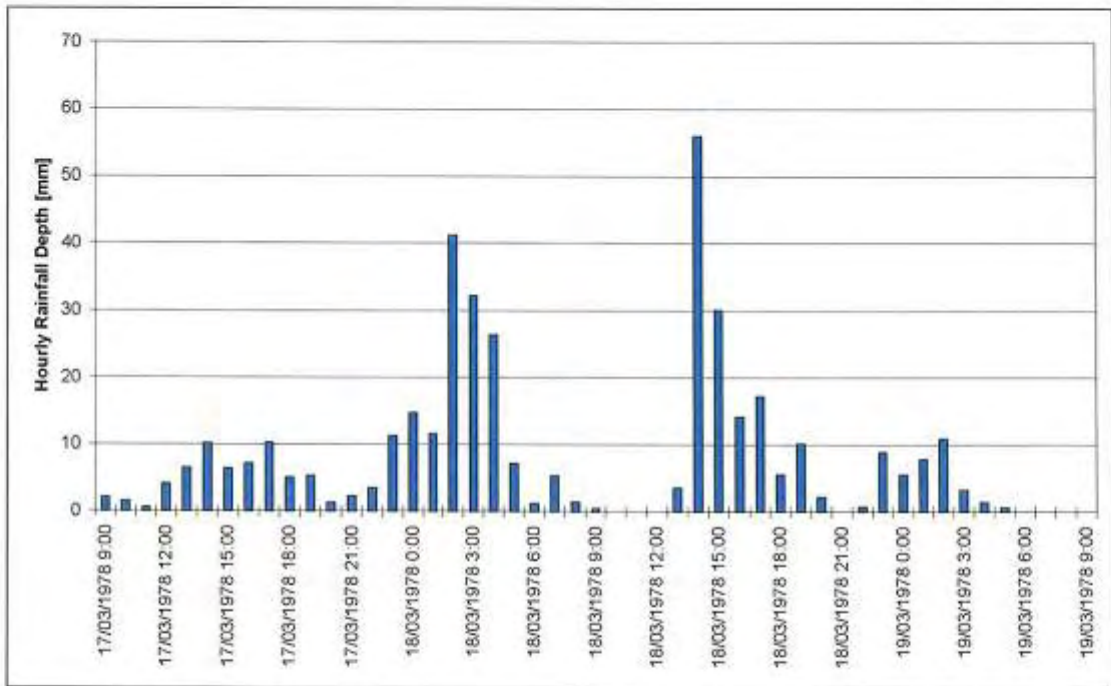
Figure 4-13 Coolangatta Bowls Comp Pluviometer, March 1978
