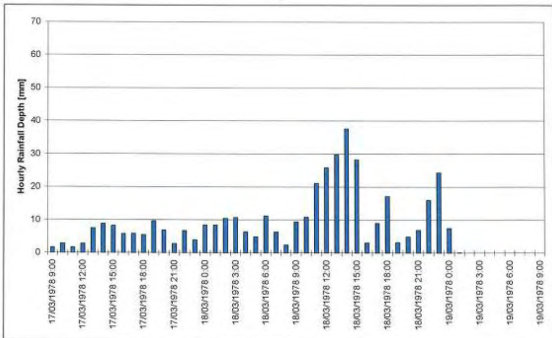
Figure 4-18 Eungella Pluviometer, March 1978
