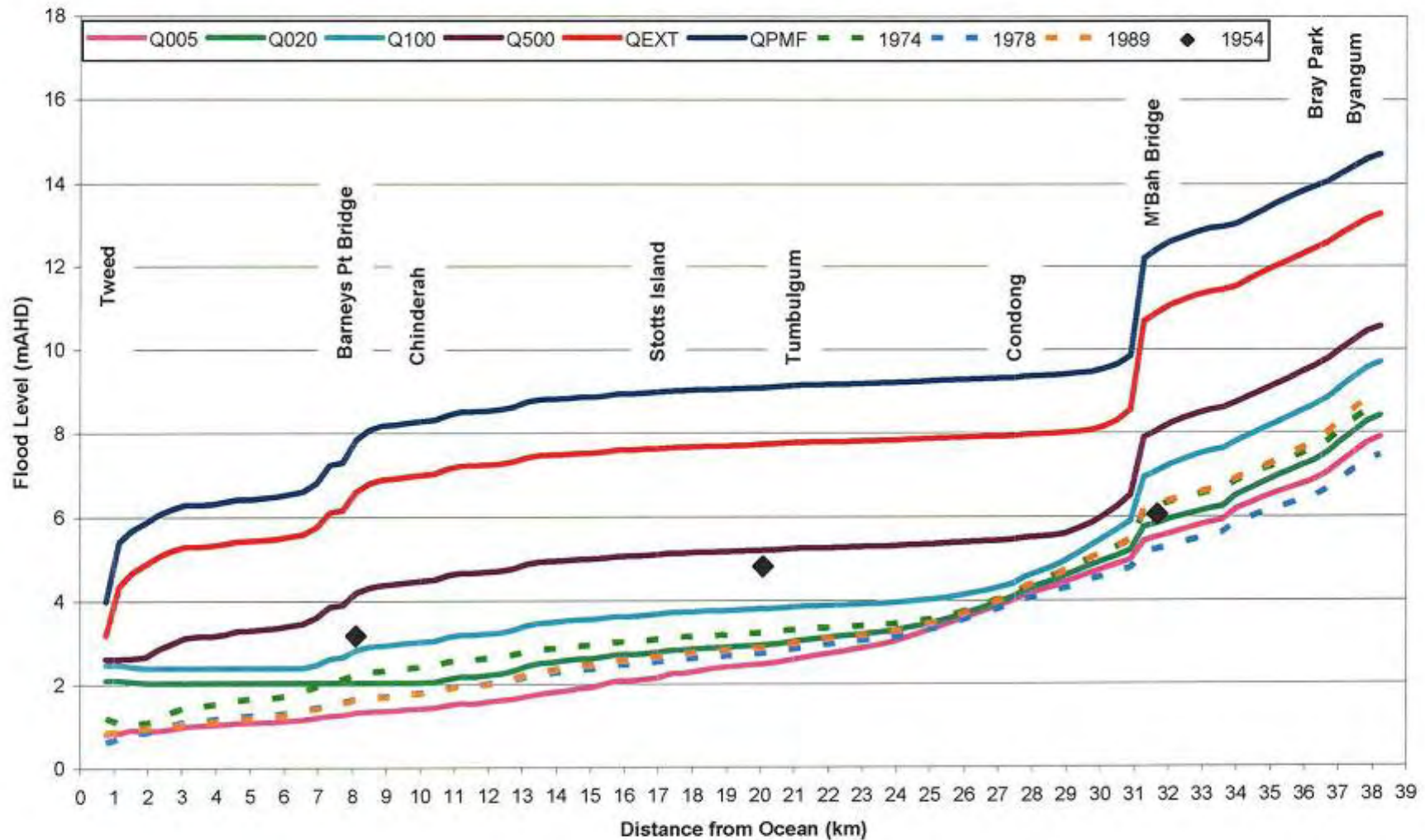
Figure 6-31 Design and Historical Flood Profiles for the Tweed River
