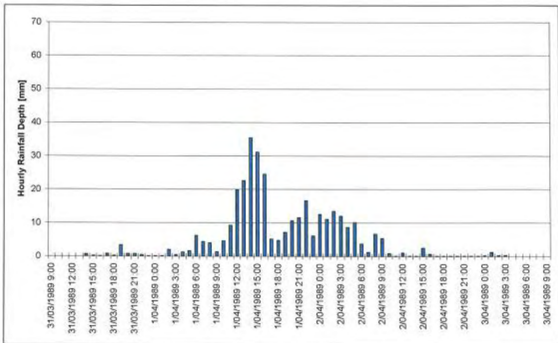
Figure 4-26 Green Pigeon Pluviometer, April 1989
