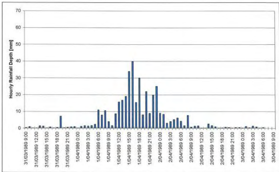
Figure 4-27 Kunghur Pluviometer, April 1989
