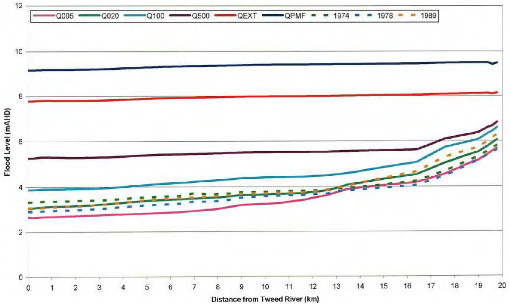
Figure 6-32 Design and Historical Flood Profiles for the Rous River
