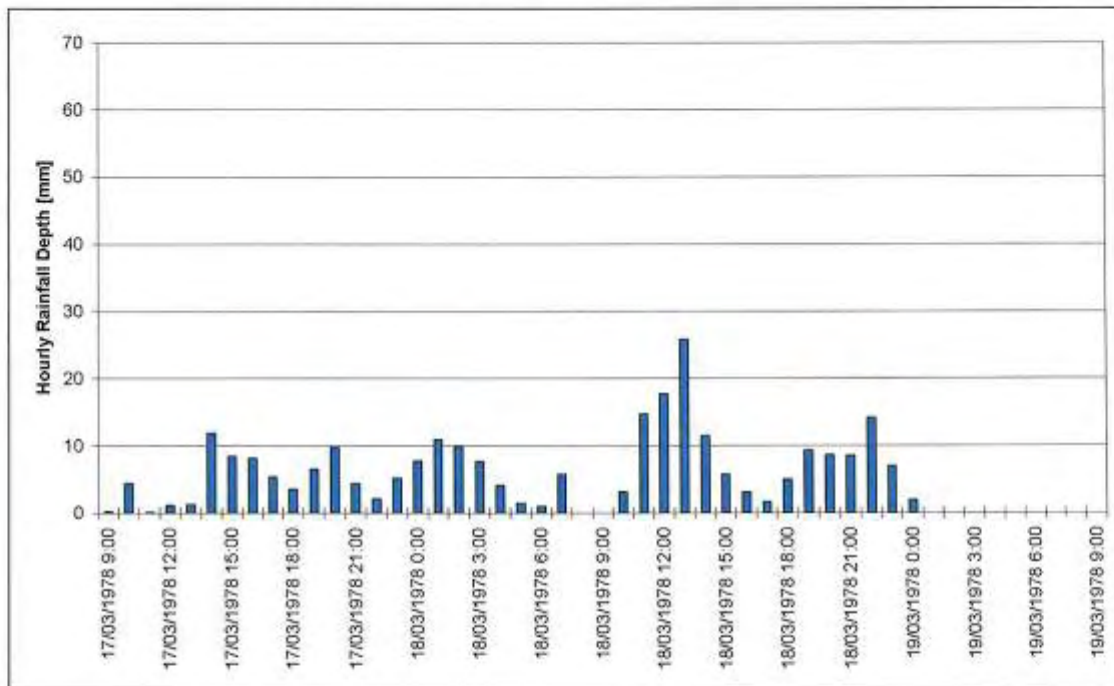
Figure 4-16 Tyalgum (Pumpenbil Rd) Pluviometer, March 1978
