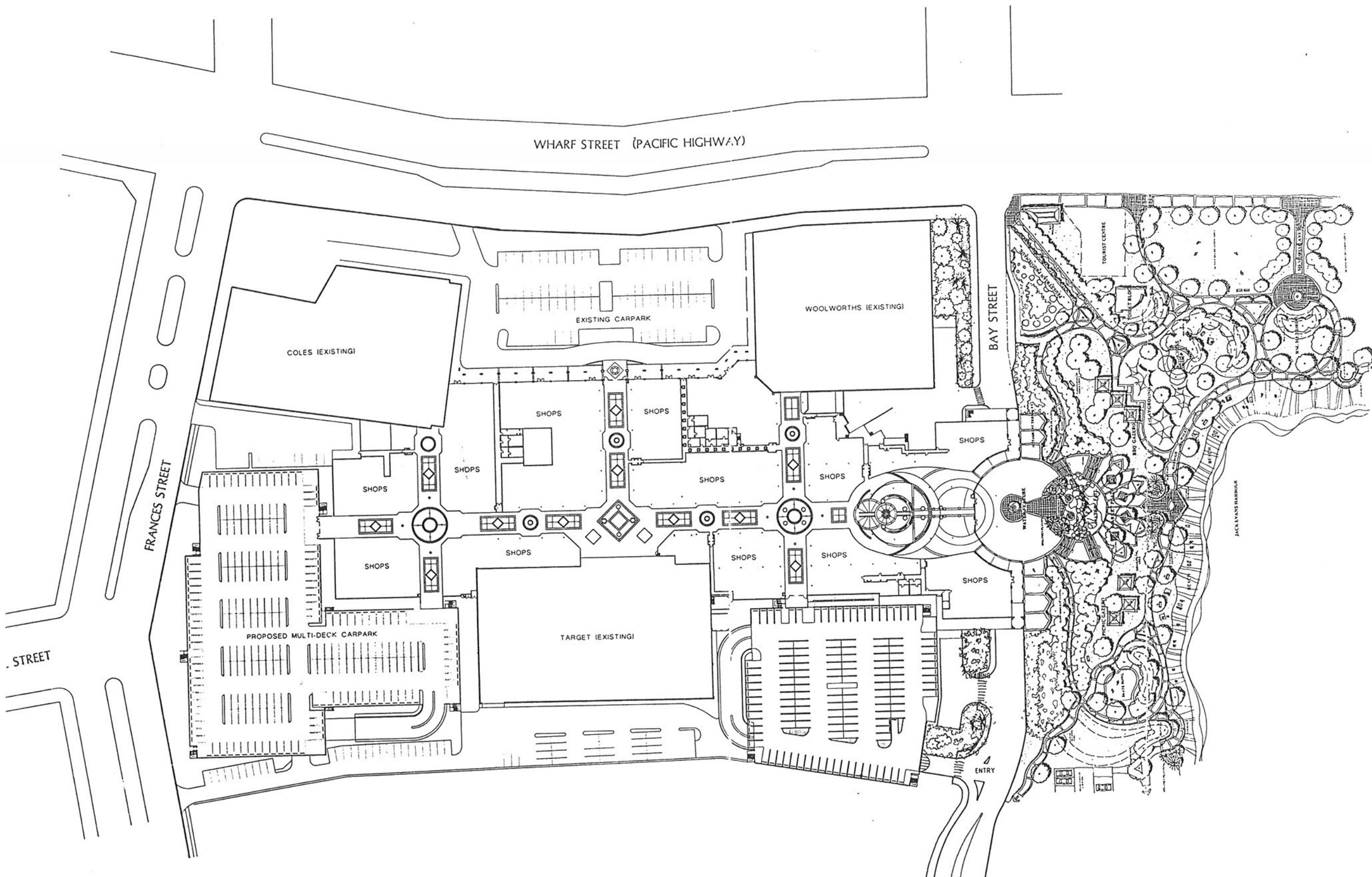
SITE PLAN 1:500 STAGE 1 & 2
