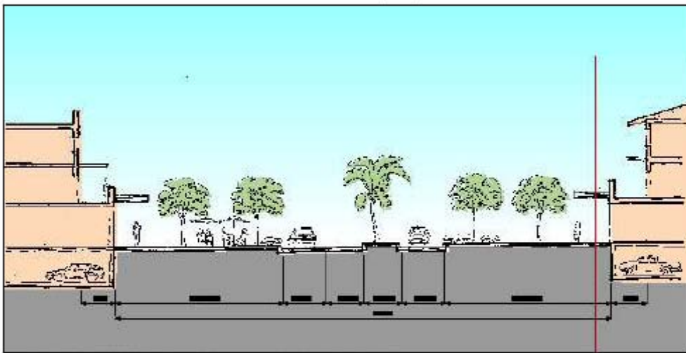
VILLAGE CENTRE Main Street Cross - section: No Parking Bays
